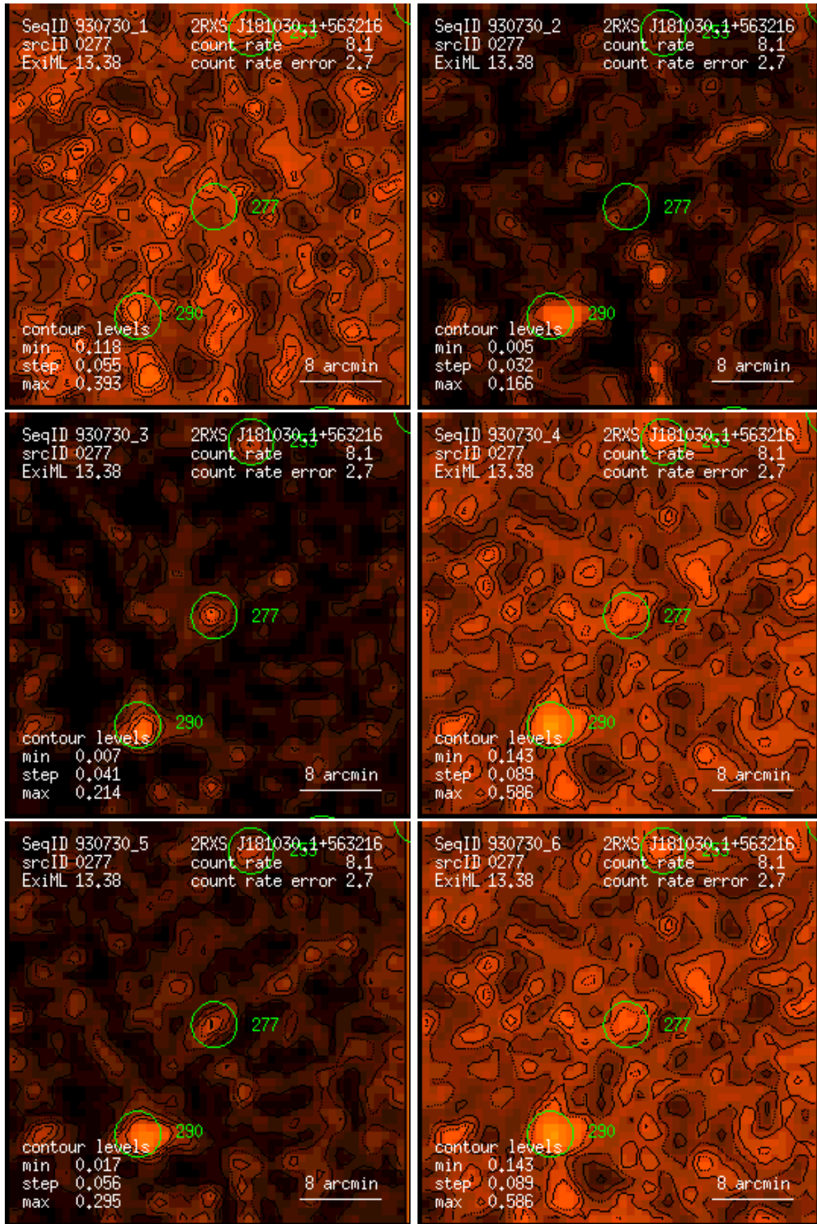
Figure 277: RASS 930730: detection 0277: band rate images, Gaussian filter: (1) PSPC channels 11 – 41, (2) 52 – 90, (3) 91 – 201, (4) 11 – 235, (5) 52 – 201, (6) 11 – 201. Broad band rates in counts/ks. Band rate contour levels in counts/ks/arcmin 2 .
