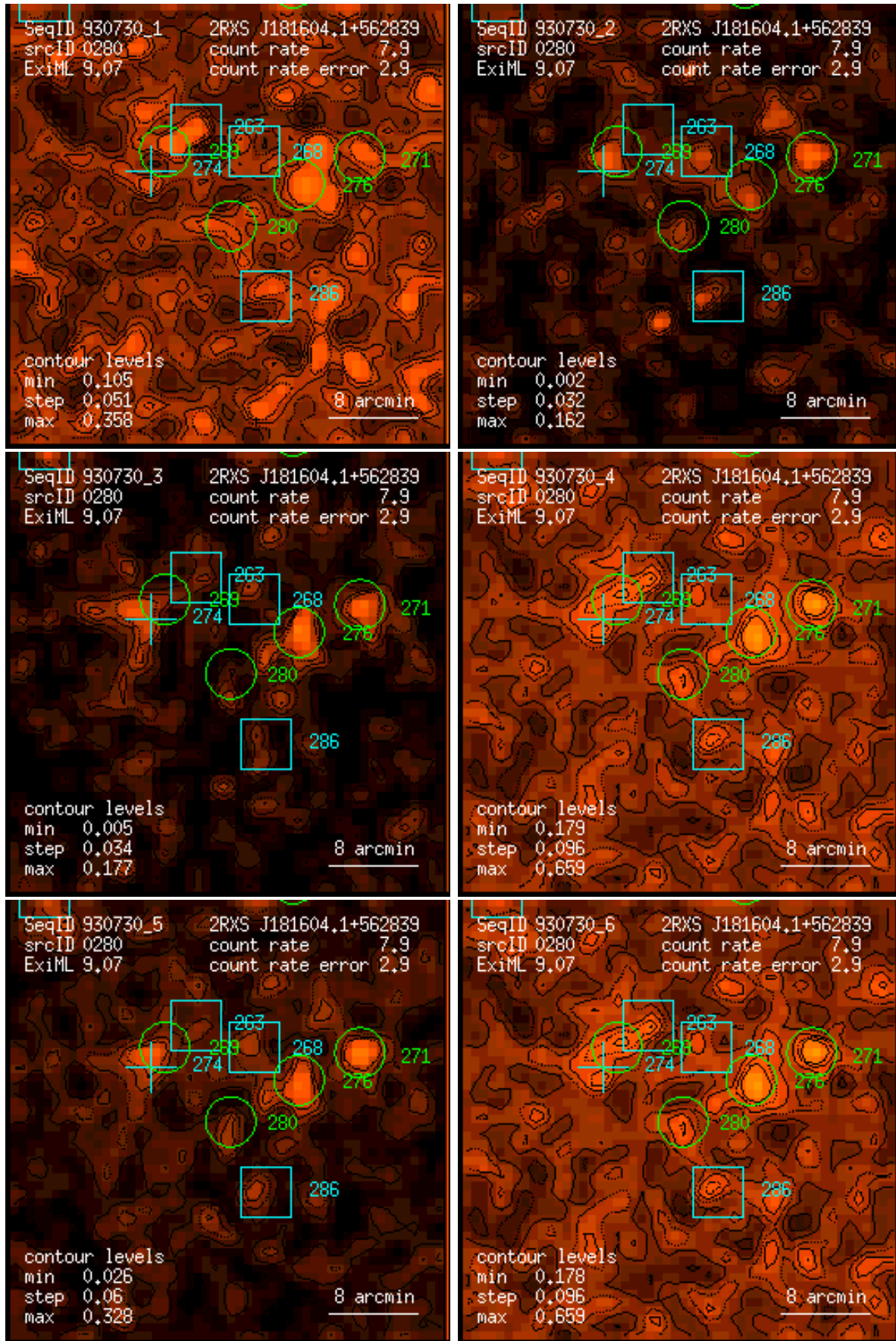
Figure 280: RASS 930730: detection 0280: band rate images, Gaussian filter: (1) PSPC channels 11 – 41, (2) 52 – 90, (3) 91 – 201, (4) 11 – 235, (5) 52 – 201, (6) 11 – 201. Broad band rates in counts/ks. Band rate contour levels in counts/ks/arcmin 2 .
