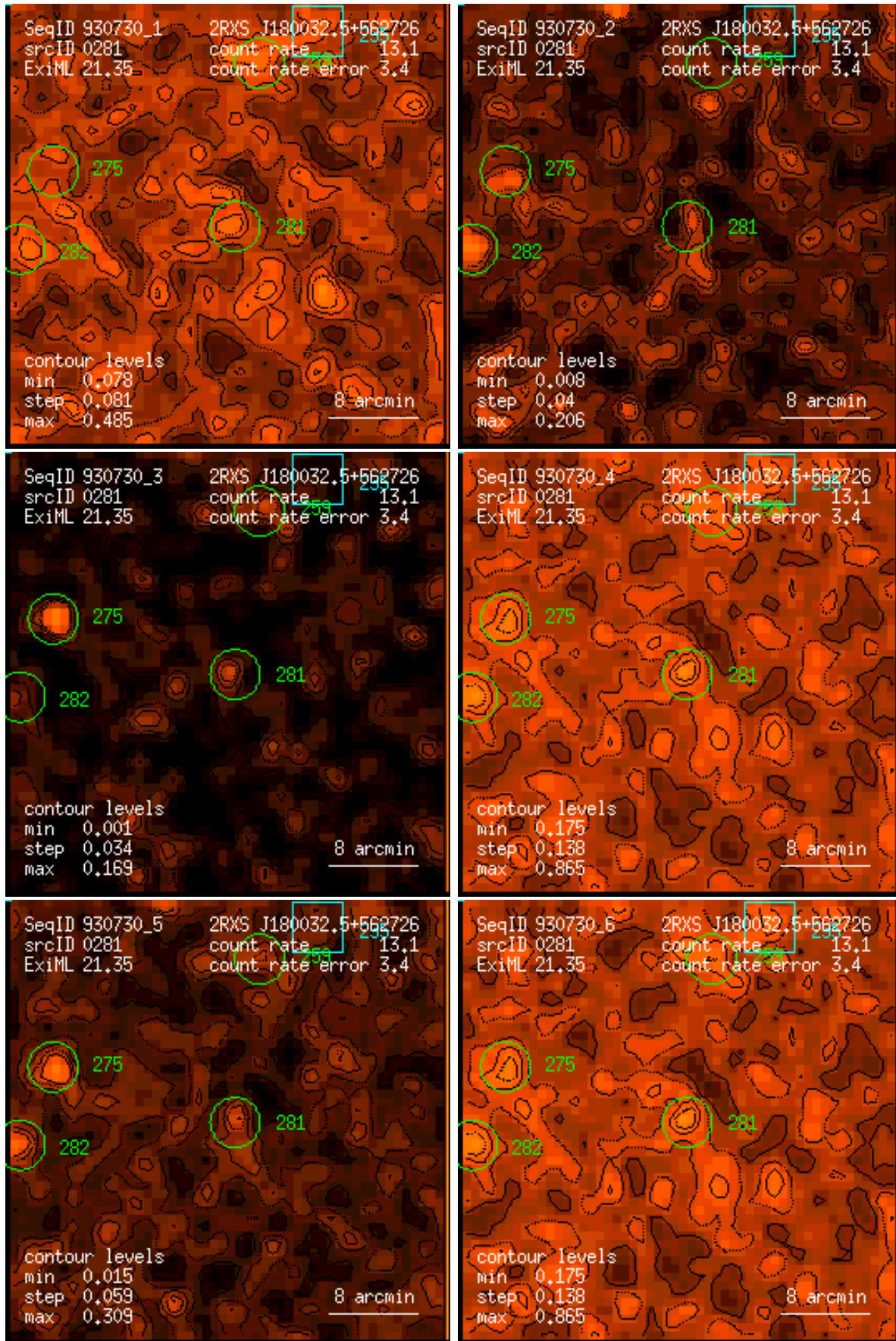
Figure 281: RASS 930730: detection 0281: band rate images, Gaussian filter: (1) PSPC channels 11 – 41, (2) 52 – 90, (3) 91 – 201, (4) 11 – 235, (5) 52 – 201, (6) 11 – 201. Broad band rates in counts/ks. Band rate contour levels in counts/ks/arcmin 2 .
