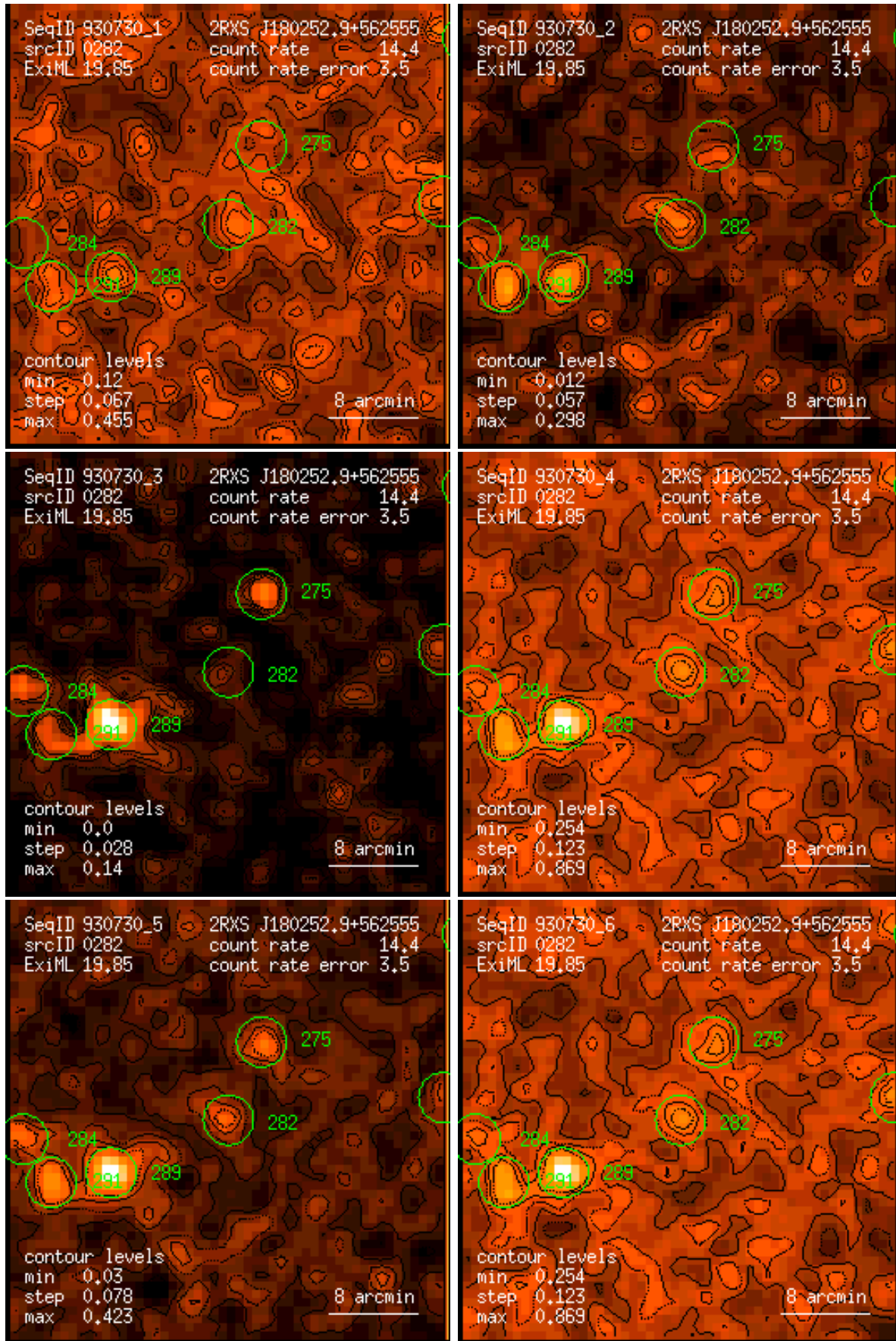
Figure 282: RASS 930730: detection 0282: band rate images, Gaussian filter: (1) PSPC channels 11 – 41, (2) 52 – 90, (3) 91 – 201, (4) 11 – 235, (5) 52 – 201, (6) 11 – 201. Broad band rates in counts/ks. Band rate contour levels in counts/ks/arcmin 2 .
