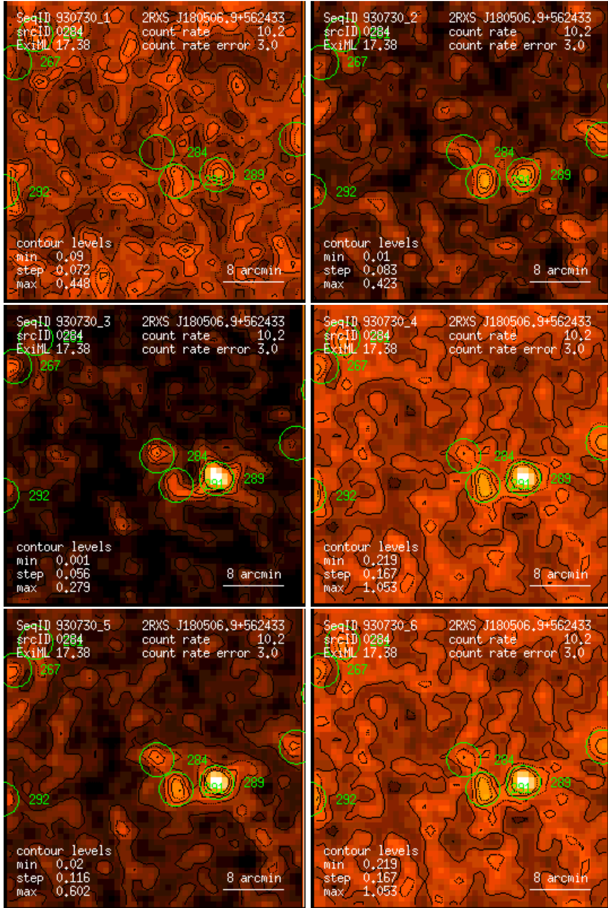
Figure 284: RASS 930730: detection 0284: band rate images, Gaussian filter: (1) PSPC channels 11 – 41, (2) 52 – 90, (3) 91 – 201, (4) 11 – 235, (5) 52 – 201, (6) 11 – 201. Broad band rates in counts/ks. Band rate contour levels in counts/ks/arcmin 2 .
