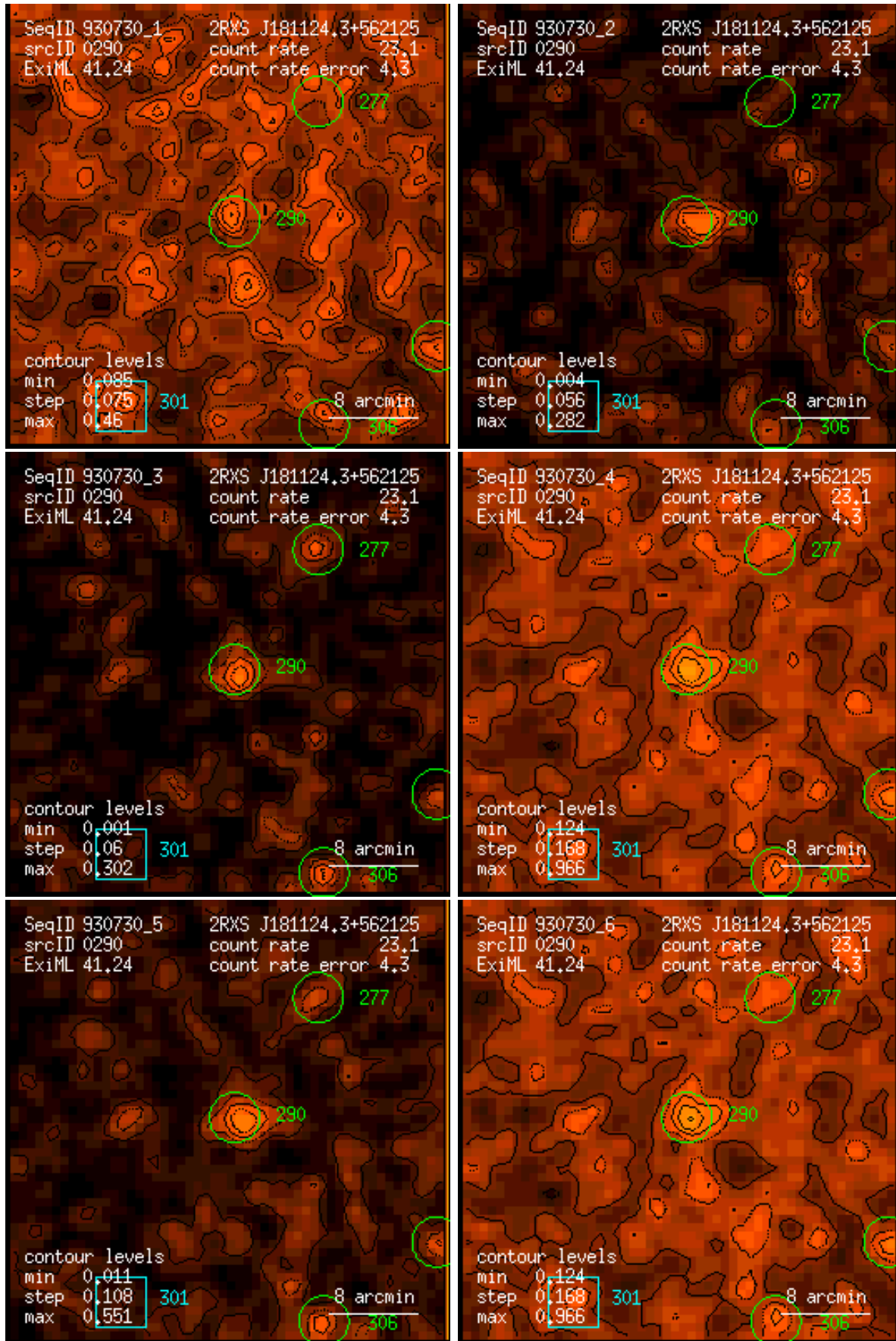
Figure 290: RASS 930730: detection 0290: band rate images, Gaussian filter: (1) PSPC channels 11 – 41, (2) 52 – 90, (3) 91 – 201, (4) 11 – 235, (5) 52 – 201, (6) 11 – 201. Broad band rates in counts/ks. Band rate contour levels in counts/ks/arcmin 2 .
