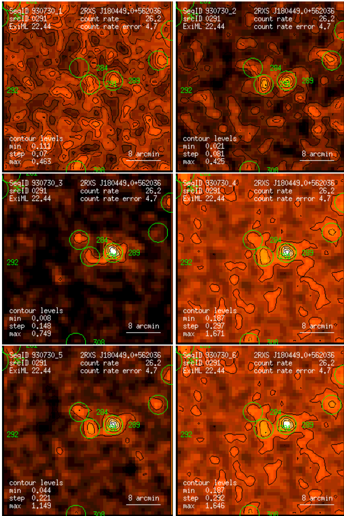
Figure 291: RASS 930730: detection 0291: band rate images, Gaussian filter: (1) PSPC channels 11 – 41, (2) 52 – 90, (3) 91 – 201, (4) 11 – 235, (5) 52 – 201, (6) 11 – 201. Broad band rates in counts/ks. Band rate contour levels in counts/ks/arcmin 2 .
