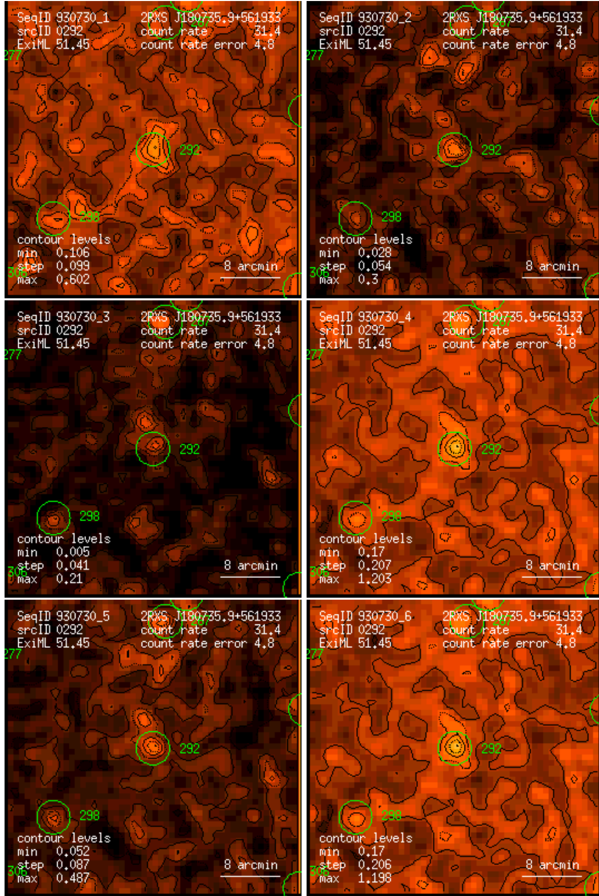
Figure 292: RASS 930730: detection 0292: band rate images, Gaussian filter: (1) PSPC channels 11 – 41, (2) 52 – 90, (3) 91 – 201, (4) 11 – 235, (5) 52 – 201, (6) 11 – 201. Broad band rates in counts/ks. Band rate contour levels in counts/ks/arcmin 2 .
