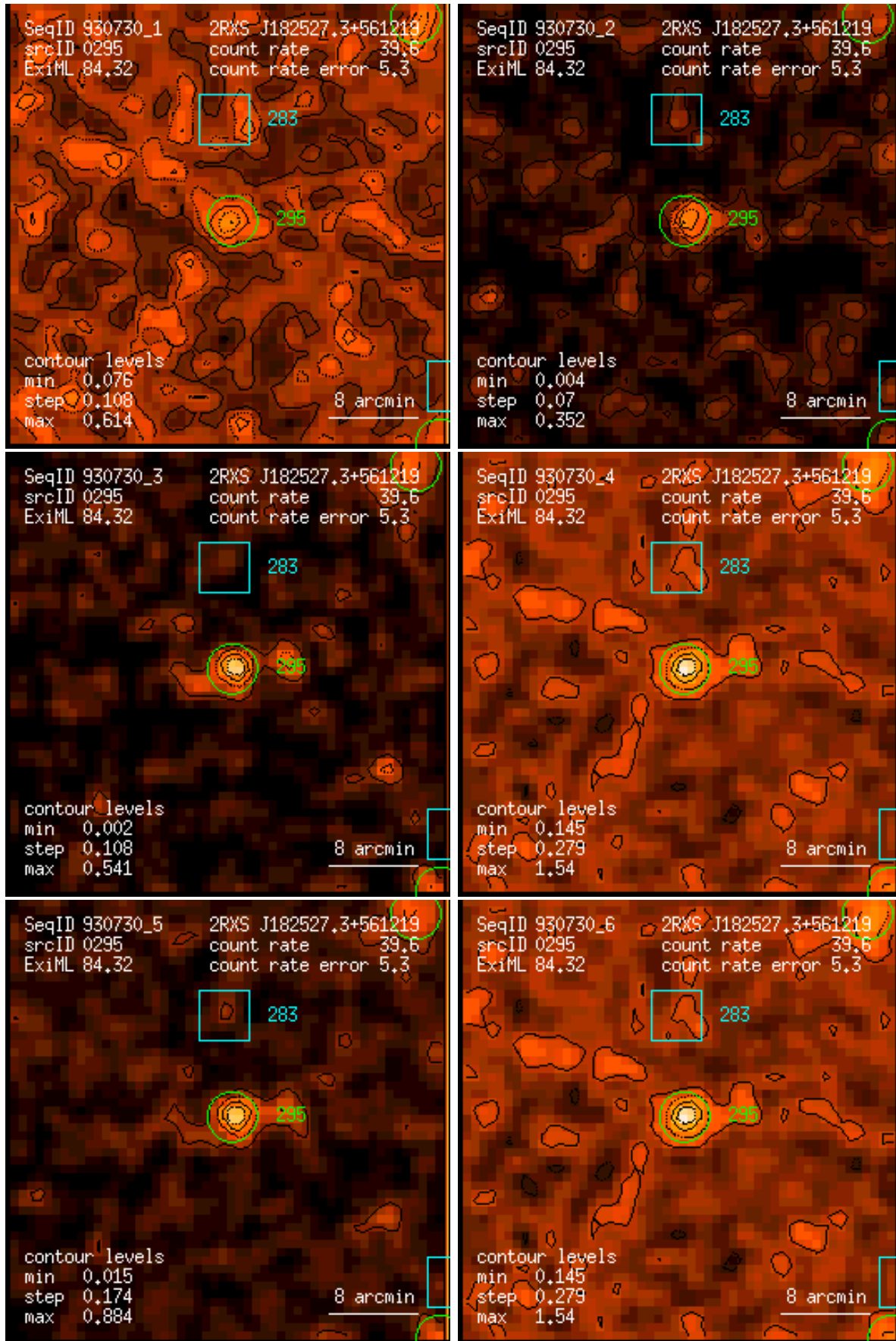
Figure 295: RASS 930730: detection 0295: band rate images, Gaussian filter: (1) PSPC channels 11 – 41, (2) 52 – 90, (3) 91 – 201, (4) 11 – 235, (5) 52 – 201, (6) 11 – 201. Broad band rates in counts/ks. Band rate contour levels in counts/ks/arcmin 2 .
