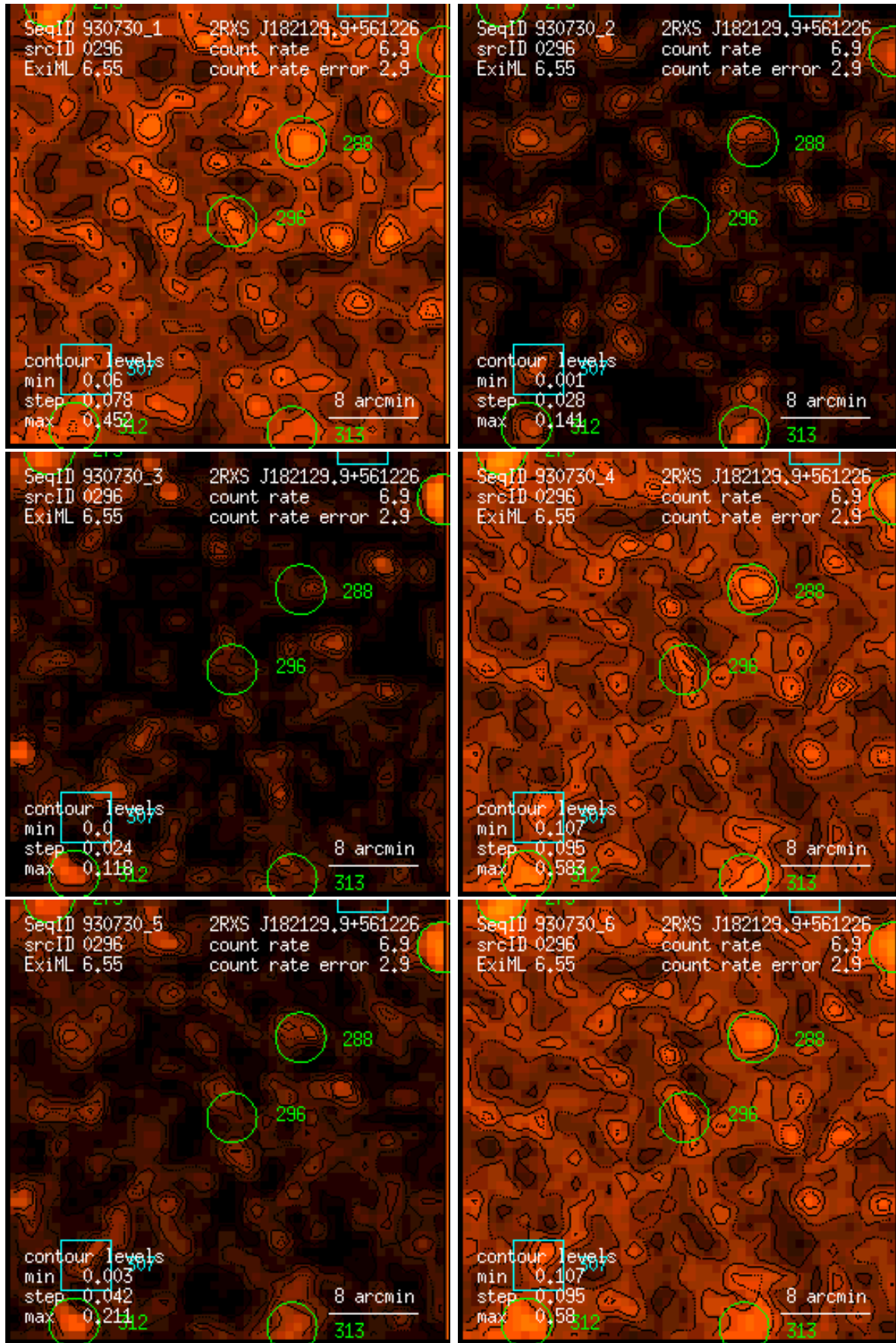
Figure 296: RASS 930730: detection 0296: band rate images, Gaussian filter: (1) PSPC channels 11 – 41, (2) 52 – 90, (3) 91 – 201, (4) 11 – 235, (5) 52 – 201, (6) 11 – 201. Broad band rates in counts/ks. Band rate contour levels in counts/ks/arcmin 2 .
