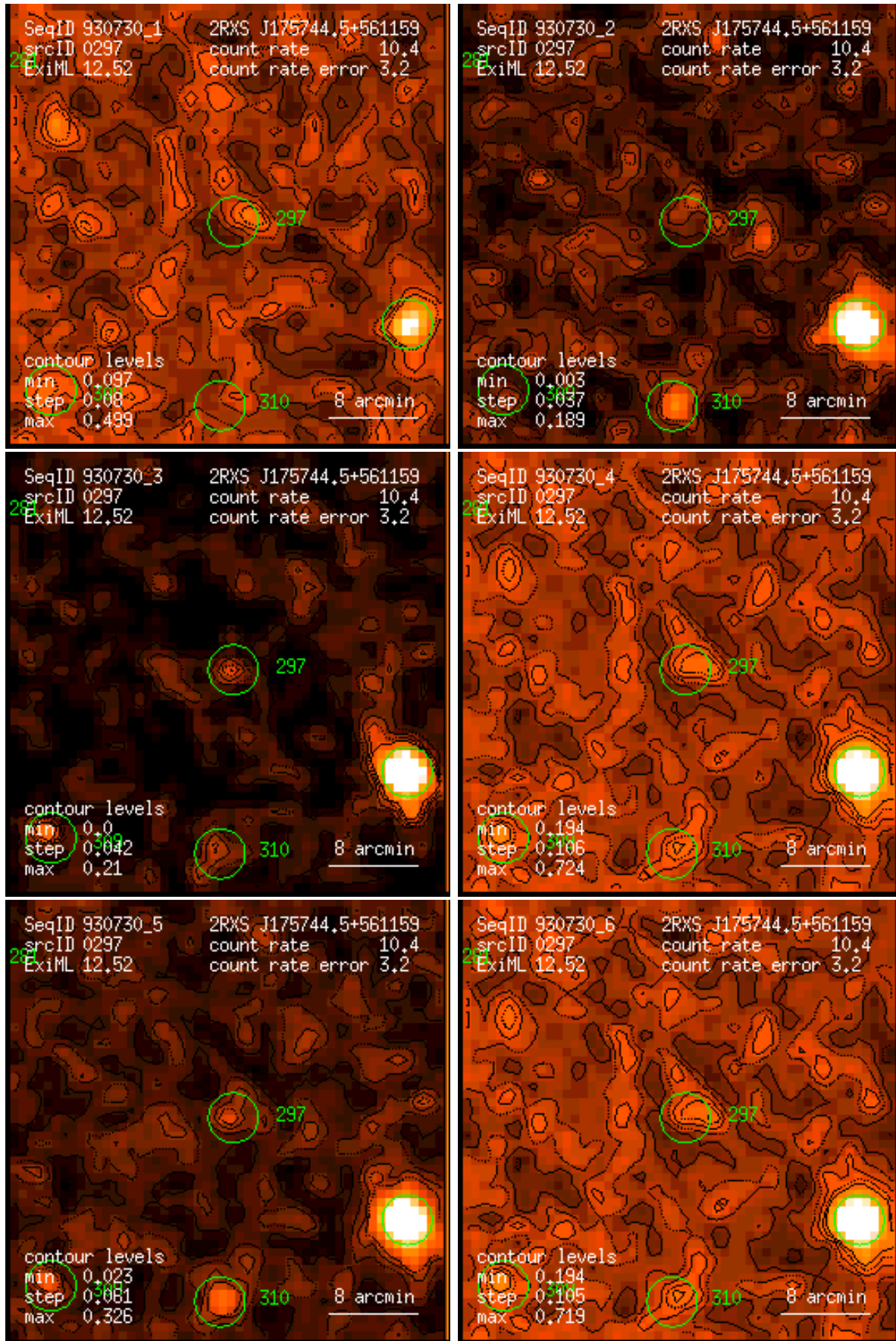
Figure 297: RASS 930730: detection 0297: band rate images, Gaussian filter: (1) PSPC channels 11 – 41, (2) 52 – 90, (3) 91 – 201, (4) 11 – 235, (5) 52 – 201, (6) 11 – 201. Broad band rates in counts/ks. Band rate contour levels in counts/ks/arcmin 2 .
