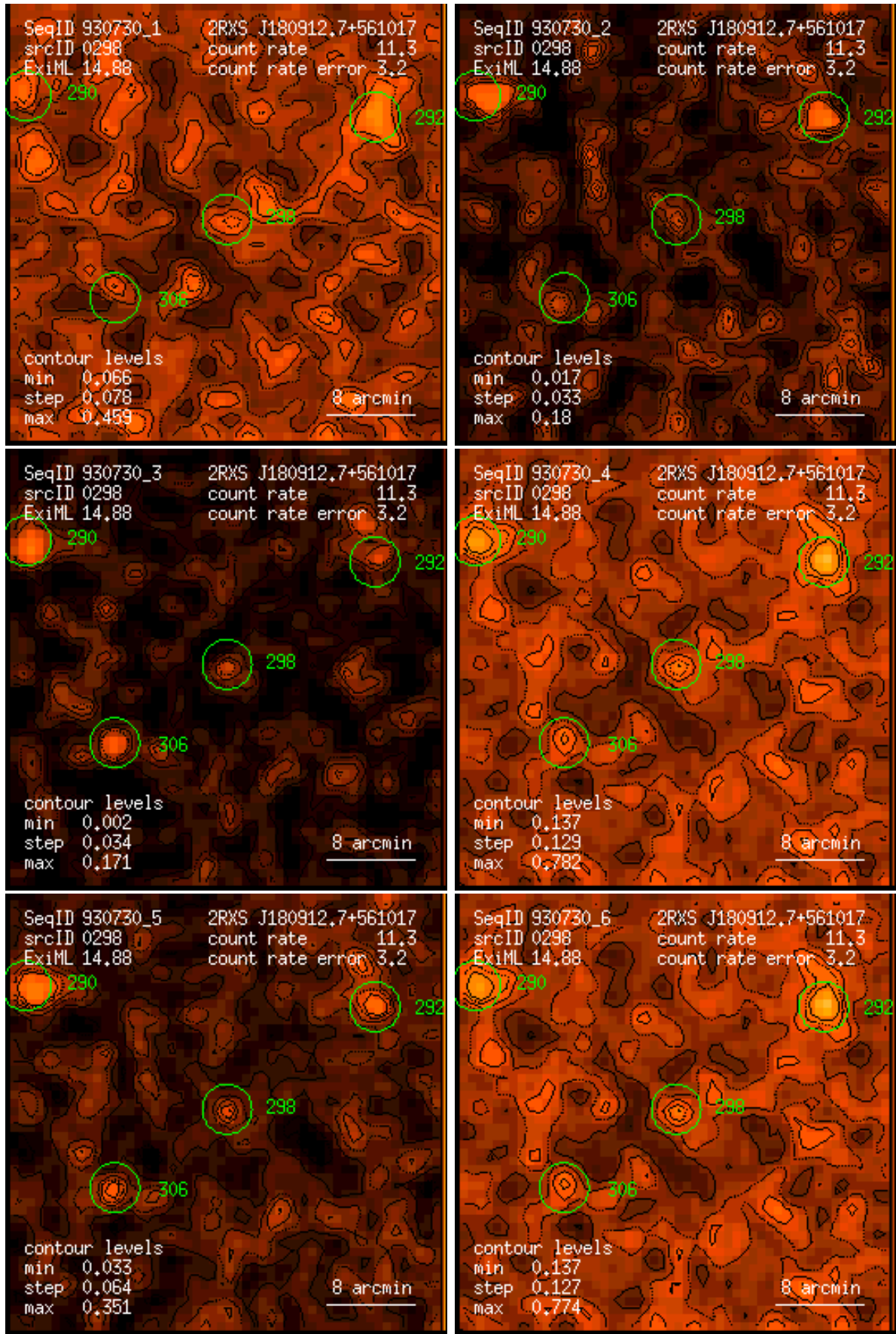
Figure 298: RASS 930730: detection 0298: band rate images, Gaussian filter: (1) PSPC channels 11 – 41, (2) 52 – 90, (3) 91 – 201, (4) 11 – 235, (5) 52 – 201, (6) 11 – 201. Broad band rates in counts/ks. Band rate contour levels in counts/ks/arcmin 2 .
