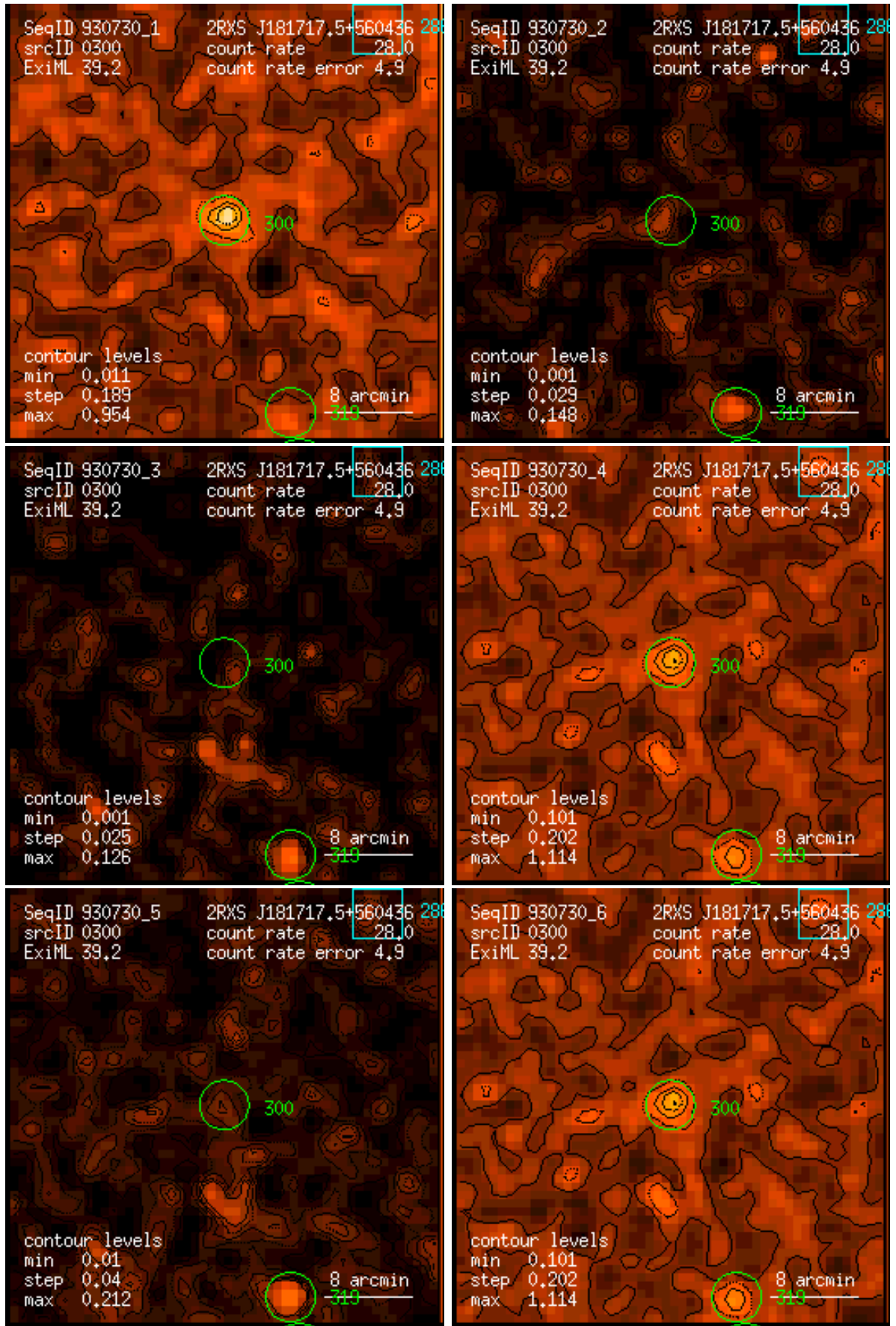
Figure 300: RASS 930730: detection 0300: band rate images, Gaussian filter: (1) PSPC channels 11 – 41, (2) 52 – 90, (3) 91 – 201, (4) 11 – 235, (5) 52 – 201, (6) 11 – 201. Broad band rates in counts/ks. Band rate contour levels in counts/ks/arcmin 2 .
