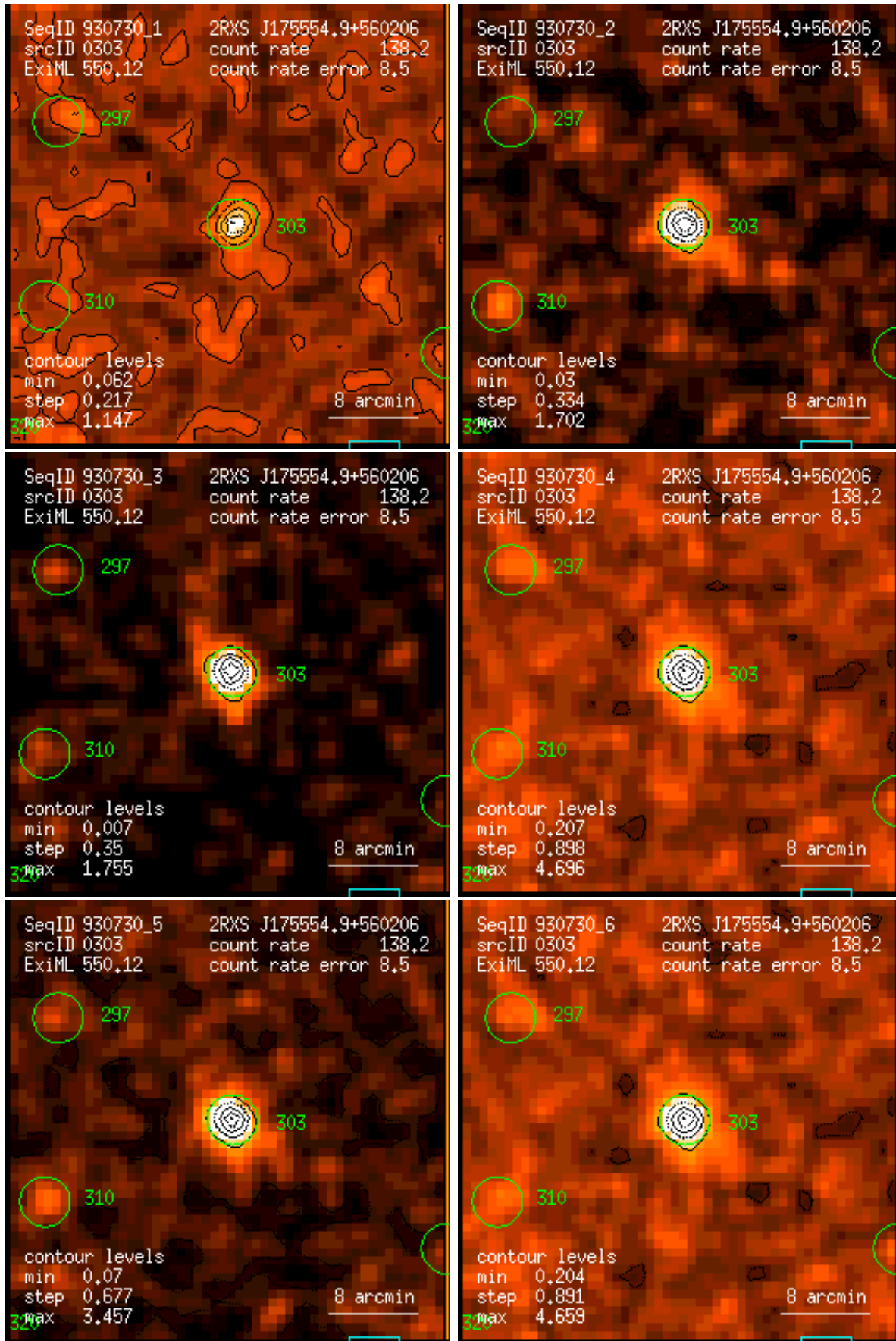
Figure 303: RASS 930730: detection 0303: band rate images, Gaussian filter: (1) PSPC channels 11 – 41, (2) 52 – 90, (3) 91 – 201, (4) 11 – 235, (5) 52 – 201, (6) 11 – 201. Broad band rates in counts/ks. Band rate contour levels in counts/ks/arcmin 2 .
