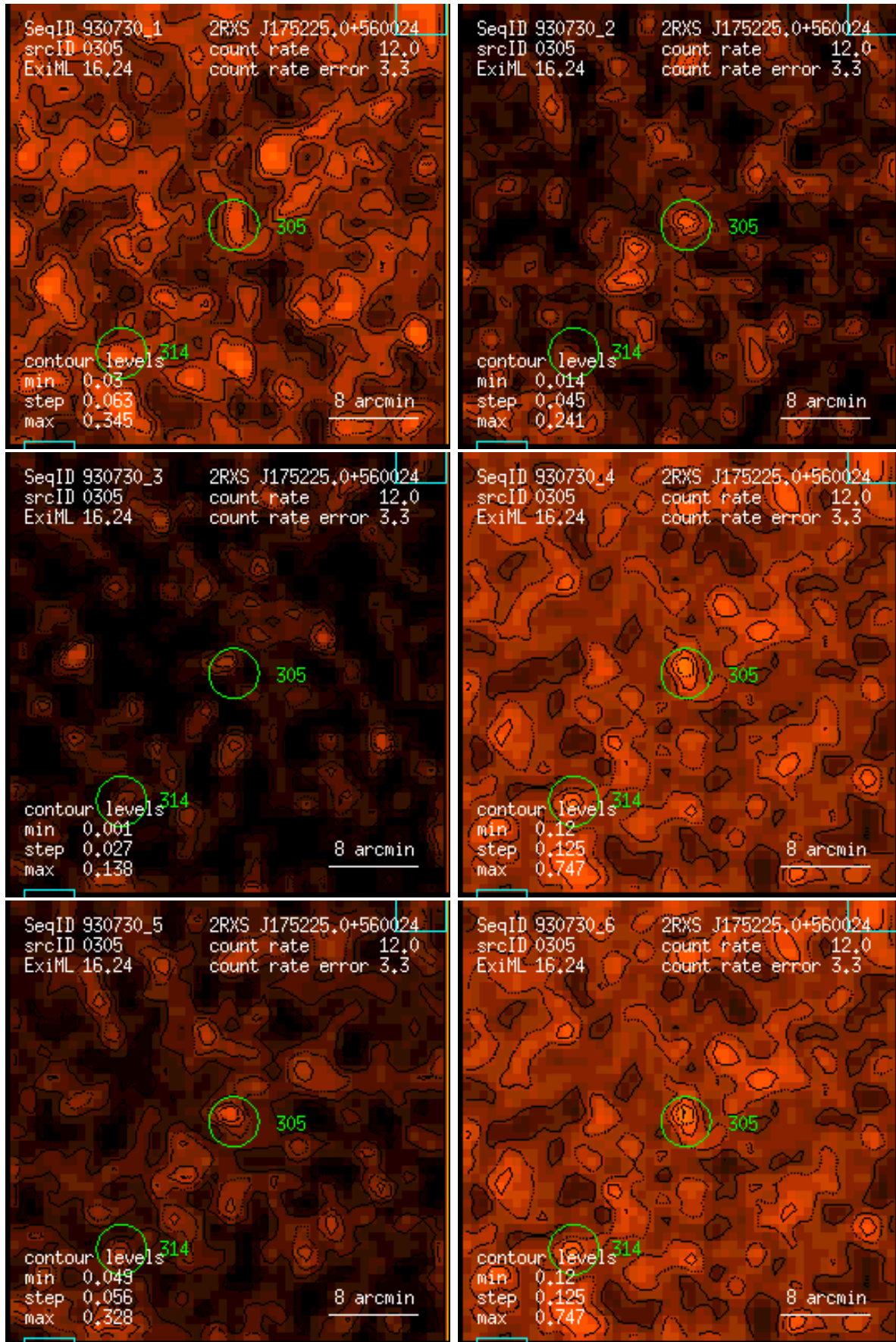
Figure 305: RASS 930730: detection 0305: band rate images, Gaussian filter: (1) PSPC channels 11 – 41, (2) 52 – 90, (3) 91 – 201, (4) 11 – 235, (5) 52 – 201, (6) 11 – 201. Broad band rates in counts/ks. Band rate contour levels in counts/ks/arcmin 2 .
