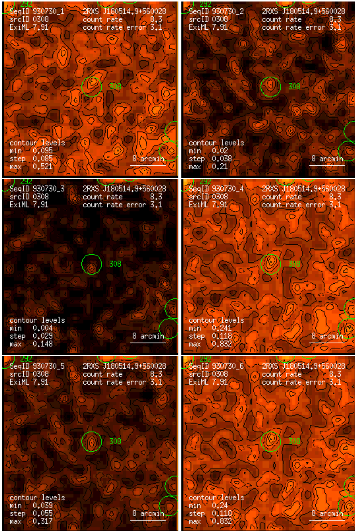
Figure 308: RASS 930730: detection 0308: band rate images, Gaussian filter: (1) PSPC channels 11 – 41, (2) 52 – 90, (3) 91 – 201, (4) 11 – 235, (5) 52 – 201, (6) 11 – 201. Broad band rates in counts/ks. Band rate contour levels in counts/ks/arcmin 2 .
