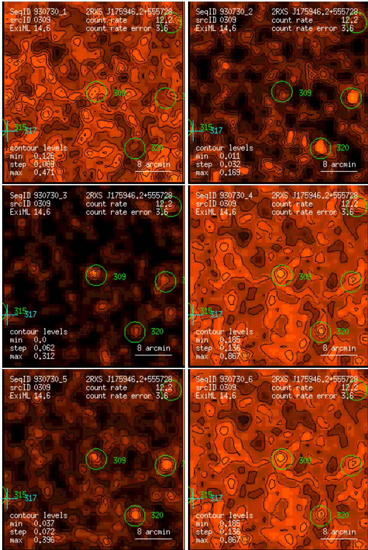
Figure 309: RASS 930730: detection 0309: band rate images, Gaussian filter: (1) PSPC channels 11 – 41, (2) 52 – 90, (3) 91 – 201, (4) 11 – 235, (5) 52 – 201, (6) 11 – 201. Broad band rates in counts/ks. Band rate contour levels in counts/ks/arcmin 2 .
