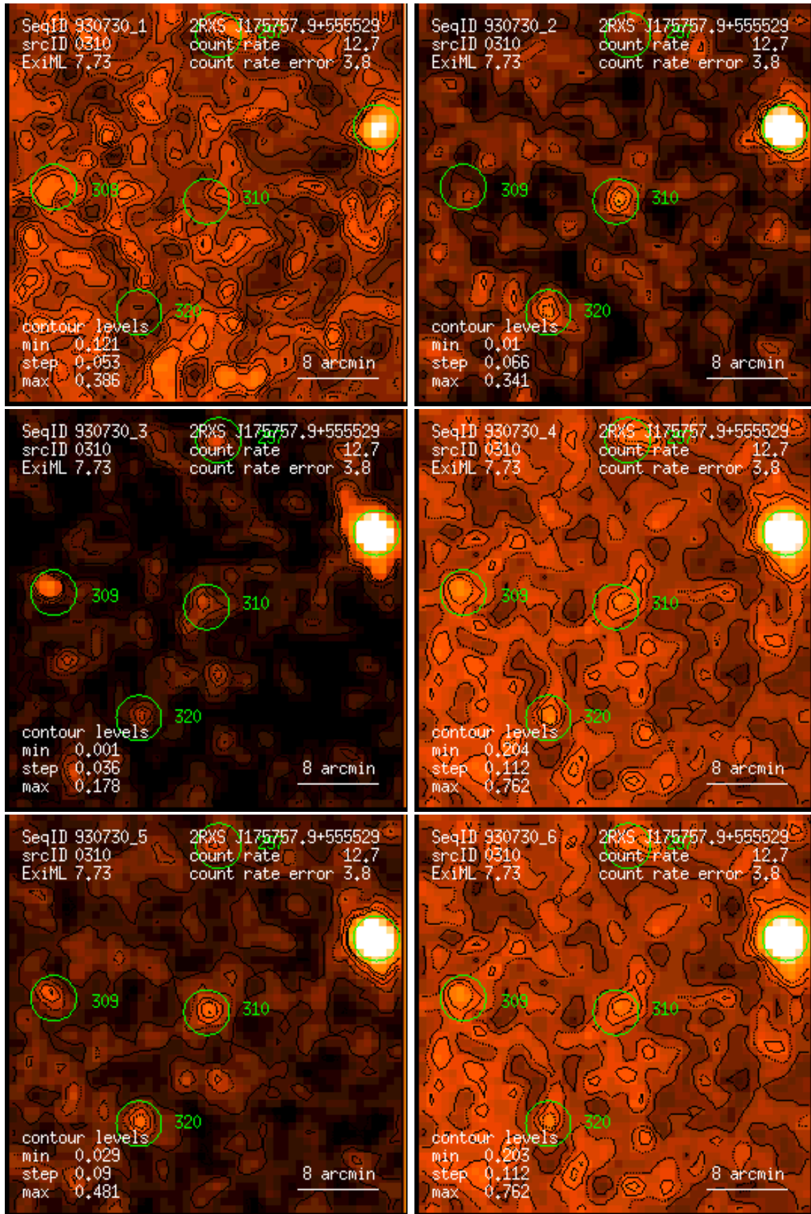
Figure 310: RASS 930730: detection 0310: band rate images, Gaussian filter: (1) PSPC channels 11 – 41, (2) 52 – 90, (3) 91 – 201, (4) 11 – 235, (5) 52 – 201, (6) 11 – 201. Broad band rates in counts/ks. Band rate contour levels in counts/ks/arcmin 2 .
