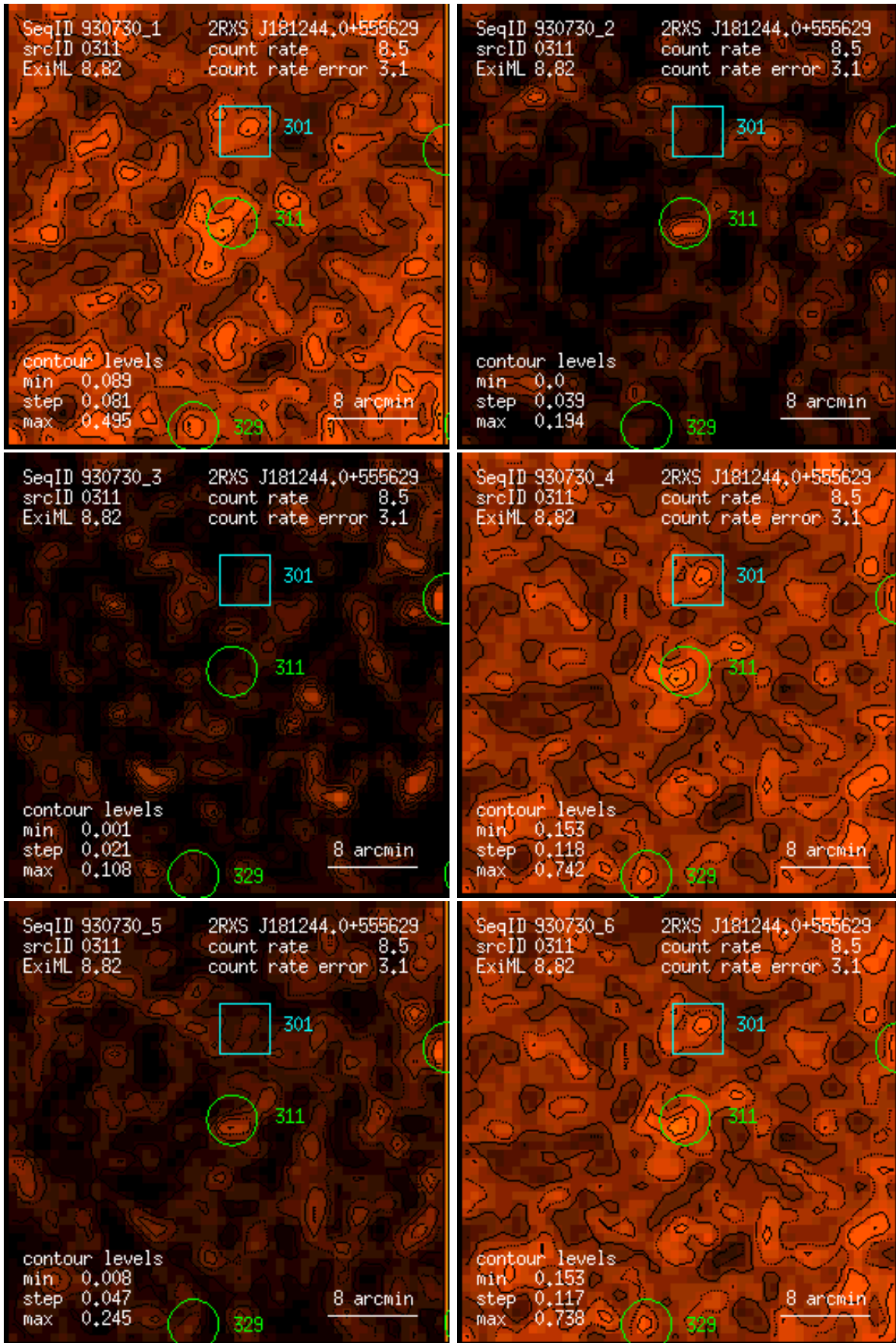
Figure 311: RASS 930730: detection 0311: band rate images, Gaussian filter: (1) PSPC channels 11 – 41, (2) 52 – 90, (3) 91 – 201, (4) 11 – 235, (5) 52 – 201, (6) 11 – 201. Broad band rates in counts/ks. Band rate contour levels in counts/ks/arcmin 2 .
