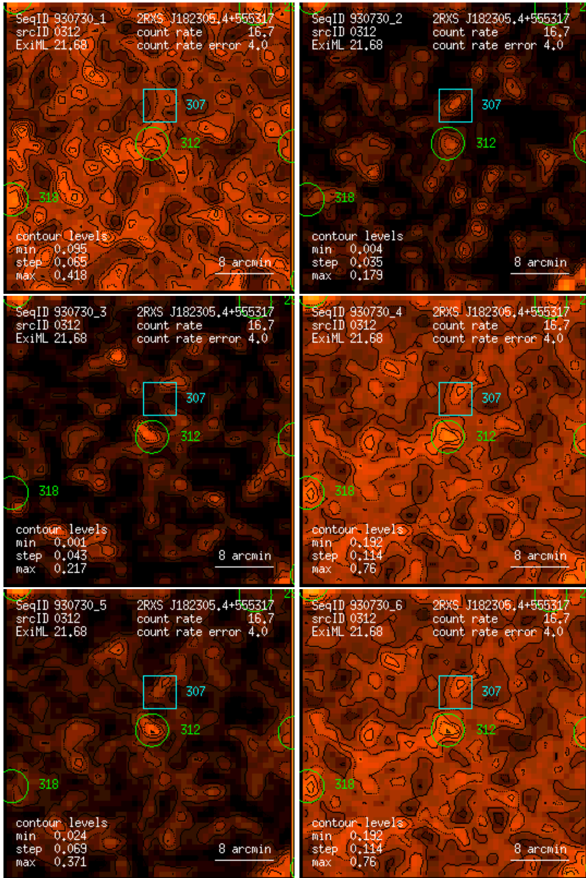
Figure 312: RASS 930730: detection 0312: band rate images, Gaussian filter: (1) PSPC channels 11 – 41, (2) 52 – 90, (3) 91 – 201, (4) 11 – 235, (5) 52 – 201, (6) 11 – 201. Broad band rates in counts/ks. Band rate contour levels in counts/ks/arcmin 2 .
