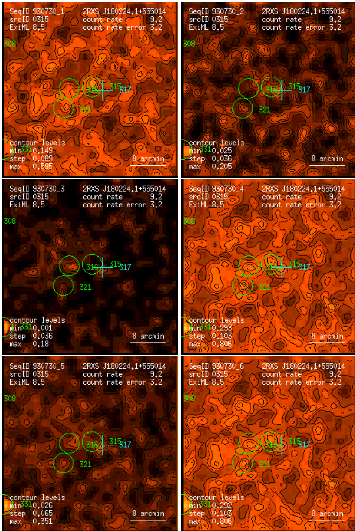
Figure 315: RASS 930730: detection 0315: band rate images, Gaussian filter: (1) PSPC channels 11 – 41, (2) 52 – 90, (3) 91 – 201, (4) 11 – 235, (5) 52 – 201, (6) 11 – 201. Broad band rates in counts/ks. Band rate contour levels in counts/ks/arcmin 2 .
