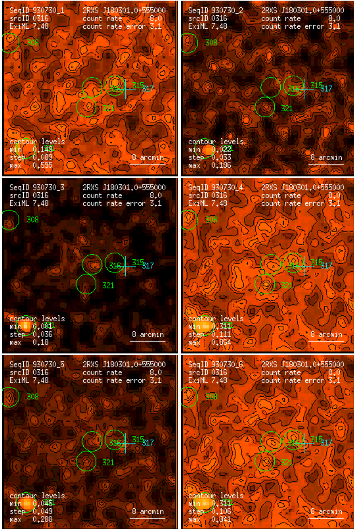
Figure 316: RASS 930730: detection 0316: band rate images, Gaussian filter: (1) PSPC channels 11 – 41, (2) 52 – 90, (3) 91 – 201, (4) 11 – 235, (5) 52 – 201, (6) 11 – 201. Broad band rates in counts/ks. Band rate contour levels in counts/ks/arcmin 2 .
