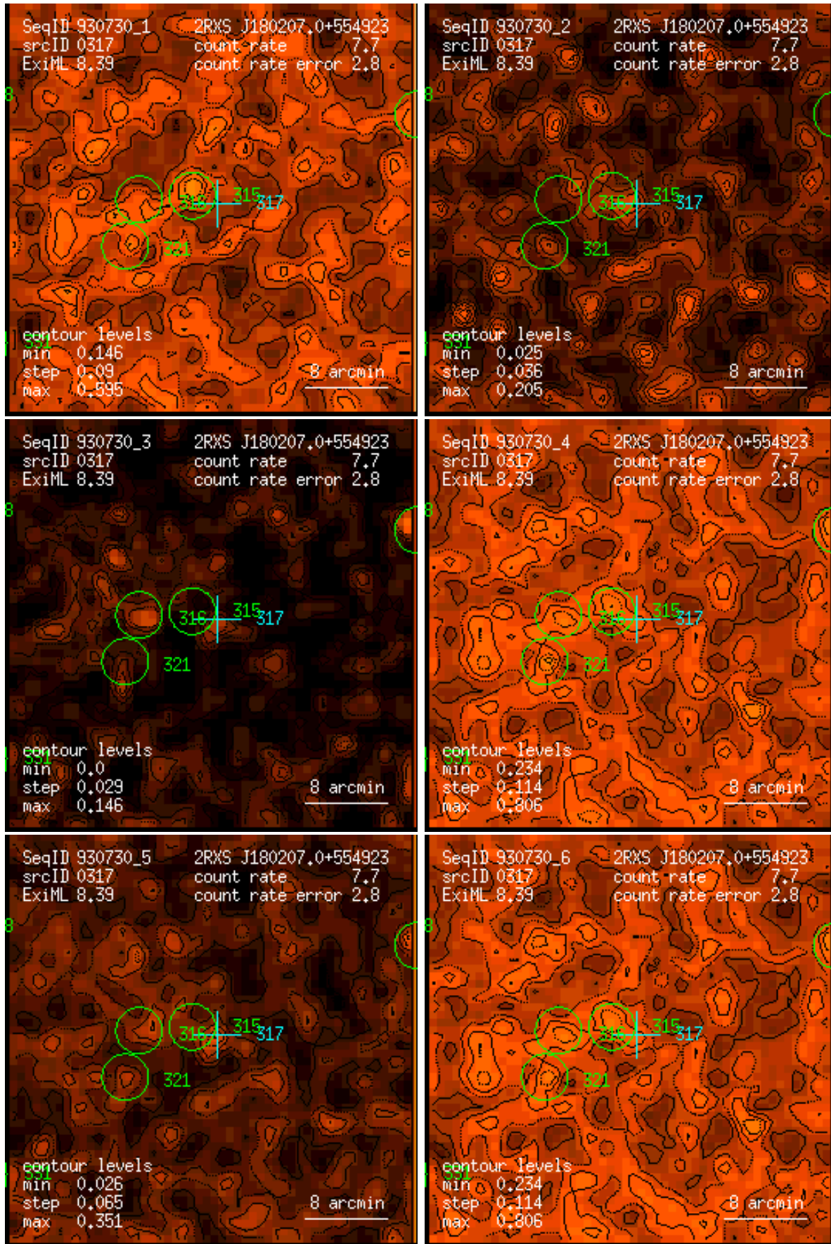
Figure 317: RASS 930730: detection 0317: band rate images, Gaussian filter: (1) PSPC channels 11 – 41, (2) 52 – 90, (3) 91 – 201, (4) 11 – 235, (5) 52 – 201, (6) 11 – 201. Broad band rates in counts/ks. Band rate contour levels in counts/ks/arcmin 2 .
