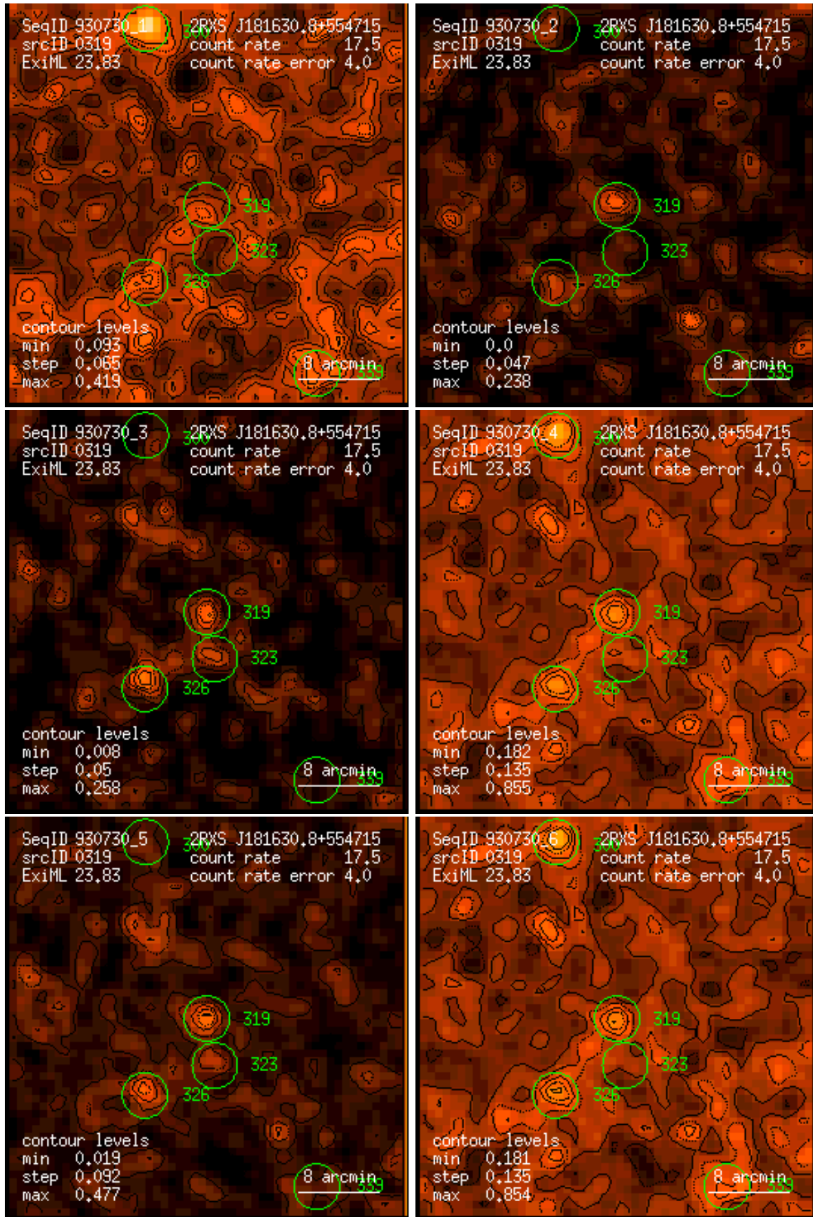
Figure 319: RASS 930730: detection 0319: band rate images, Gaussian filter: (1) PSPC channels 11 – 41, (2) 52 – 90, (3) 91 – 201, (4) 11 – 235, (5) 52 – 201, (6) 11 – 201. Broad band rates in counts/ks. Band rate contour levels in counts/ks/arcmin 2 .
