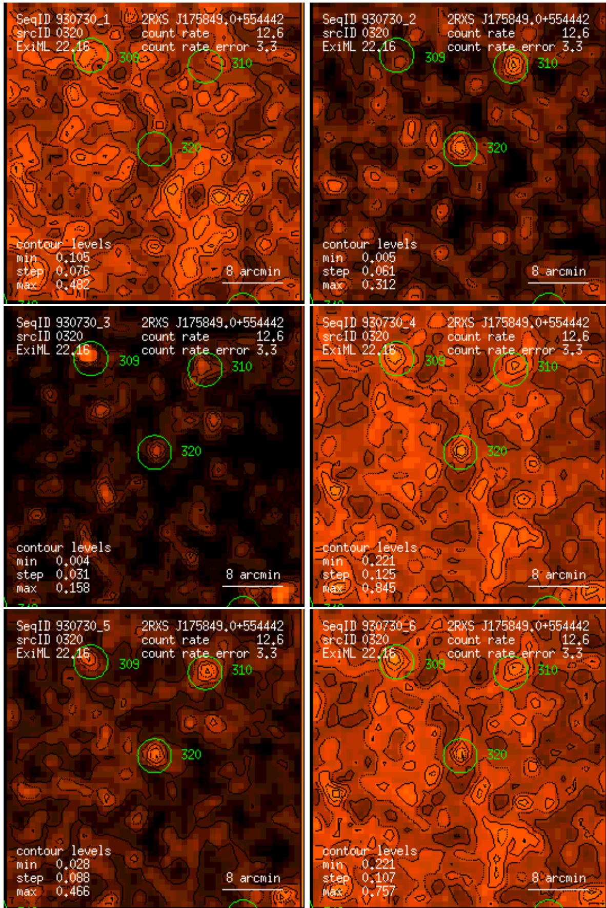
Figure 320: RASS 930730: detection 0320: band rate images, Gaussian filter: (1) PSPC channels 11 – 41, (2) 52 – 90, (3) 91 – 201, (4) 11 – 235, (5) 52 – 201, (6) 11 – 201. Broad band rates in counts/ks. Band rate contour levels in counts/ks/arcmin 2 .
