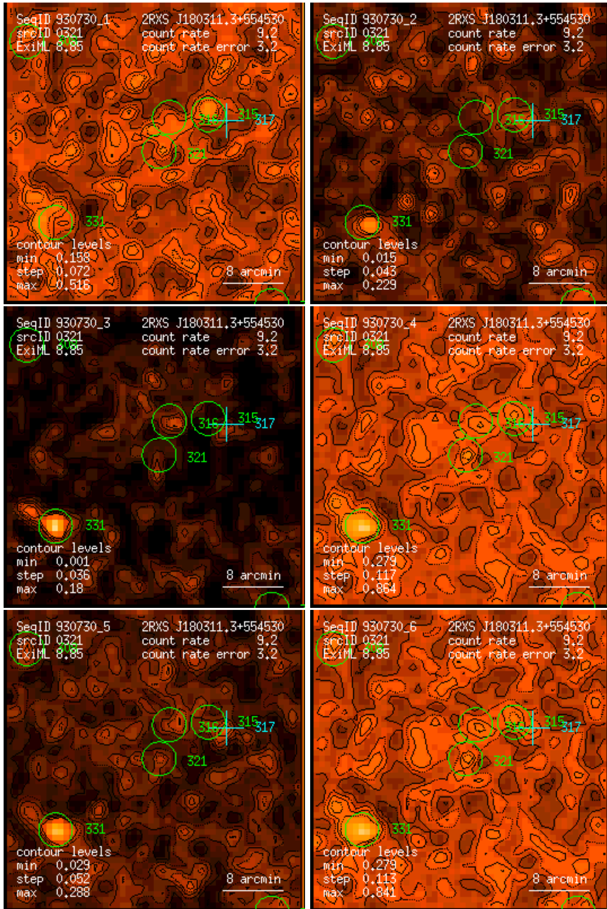
Figure 321: RASS 930730: detection 0321: band rate images, Gaussian filter: (1) PSPC channels 11 – 41, (2) 52 – 90, (3) 91 – 201, (4) 11 – 235, (5) 52 – 201, (6) 11 – 201. Broad band rates in counts/ks. Band rate contour levels in counts/ks/arcmin 2 .
