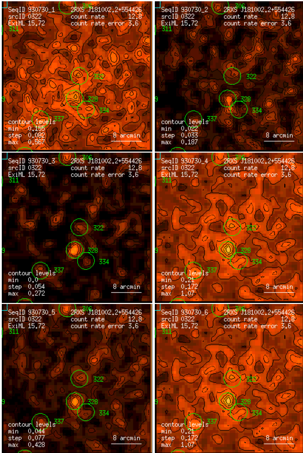
Figure 322: RASS 930730: detection 0322: band rate images, Gaussian filter: (1) PSPC channels 11 – 41, (2) 52 – 90, (3) 91 – 201, (4) 11 – 235, (5) 52 – 201, (6) 11 – 201. Broad band rates in counts/ks. Band rate contour levels in counts/ks/arcmin 2 .
