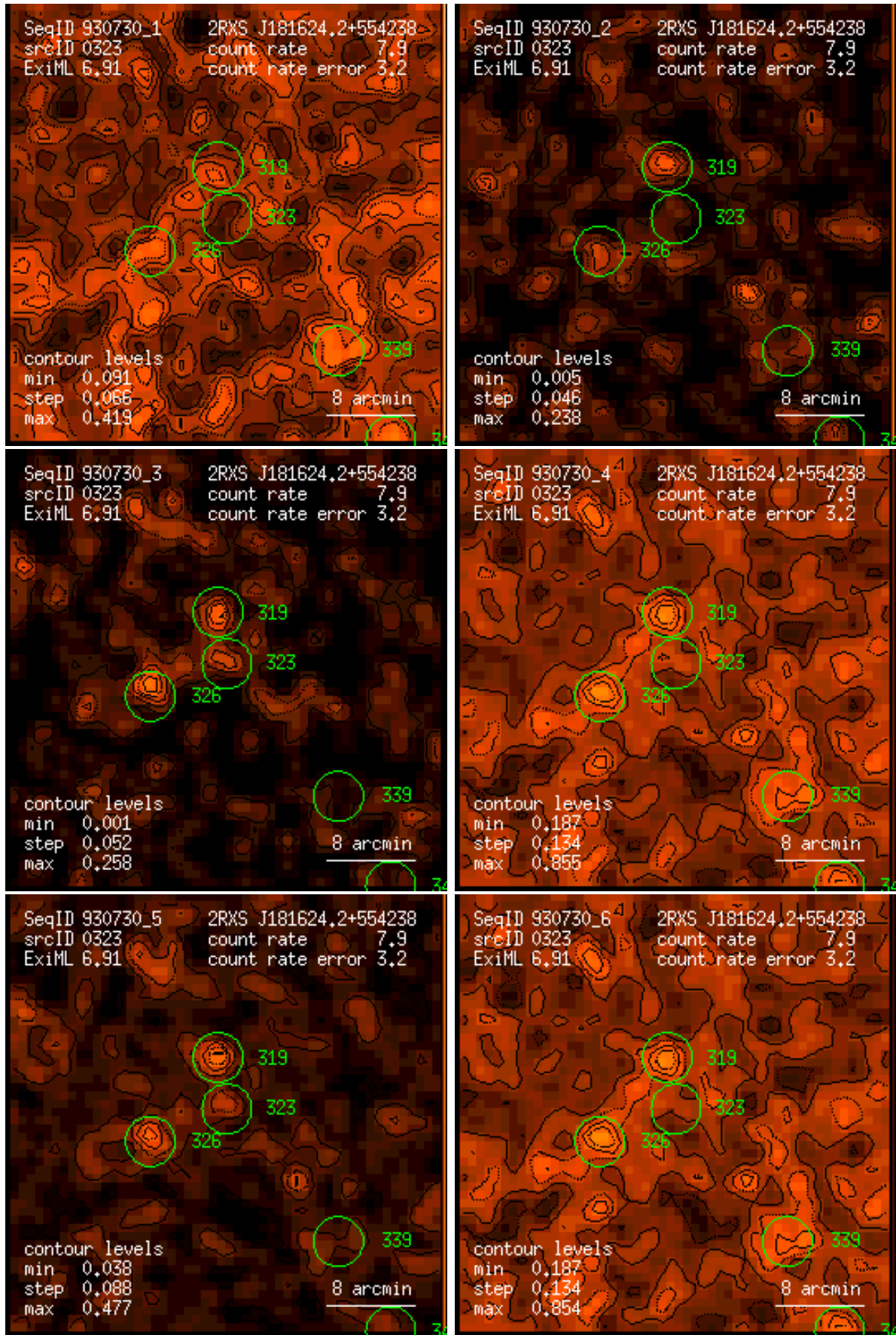
Figure 323: RASS 930730: detection 0323: band rate images, Gaussian filter: (1) PSPC channels 11 – 41, (2) 52 – 90, (3) 91 – 201, (4) 11 – 235, (5) 52 – 201, (6) 11 – 201. Broad band rates in counts/ks. Band rate contour levels in counts/ks/arcmin 2 .
