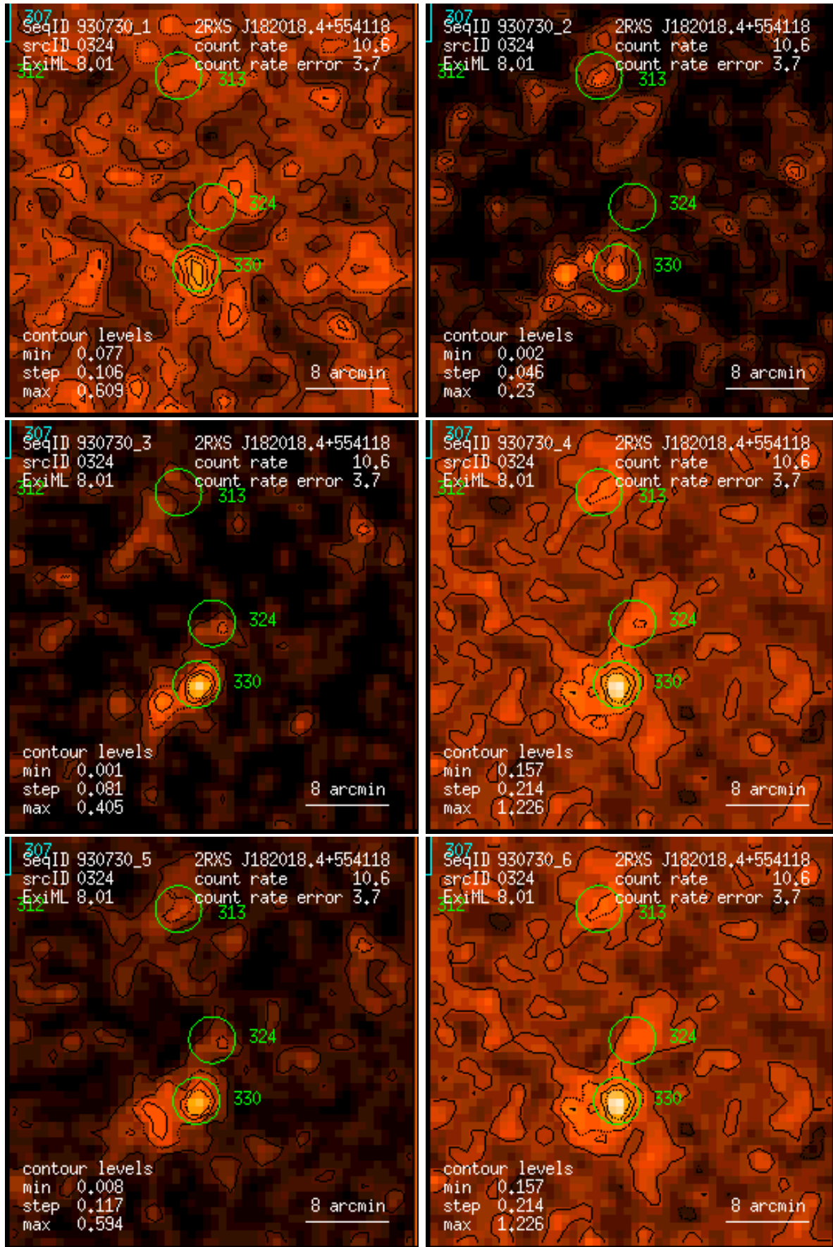
Figure 324: RASS 930730: detection 0324: band rate images, Gaussian filter: (1) PSPC channels 11 – 41, (2) 52 – 90, (3) 91 – 201, (4) 11 – 235, (5) 52 – 201, (6) 11 – 201. Broad band rates in counts/ks. Band rate contour levels in counts/ks/arcmin 2 .
