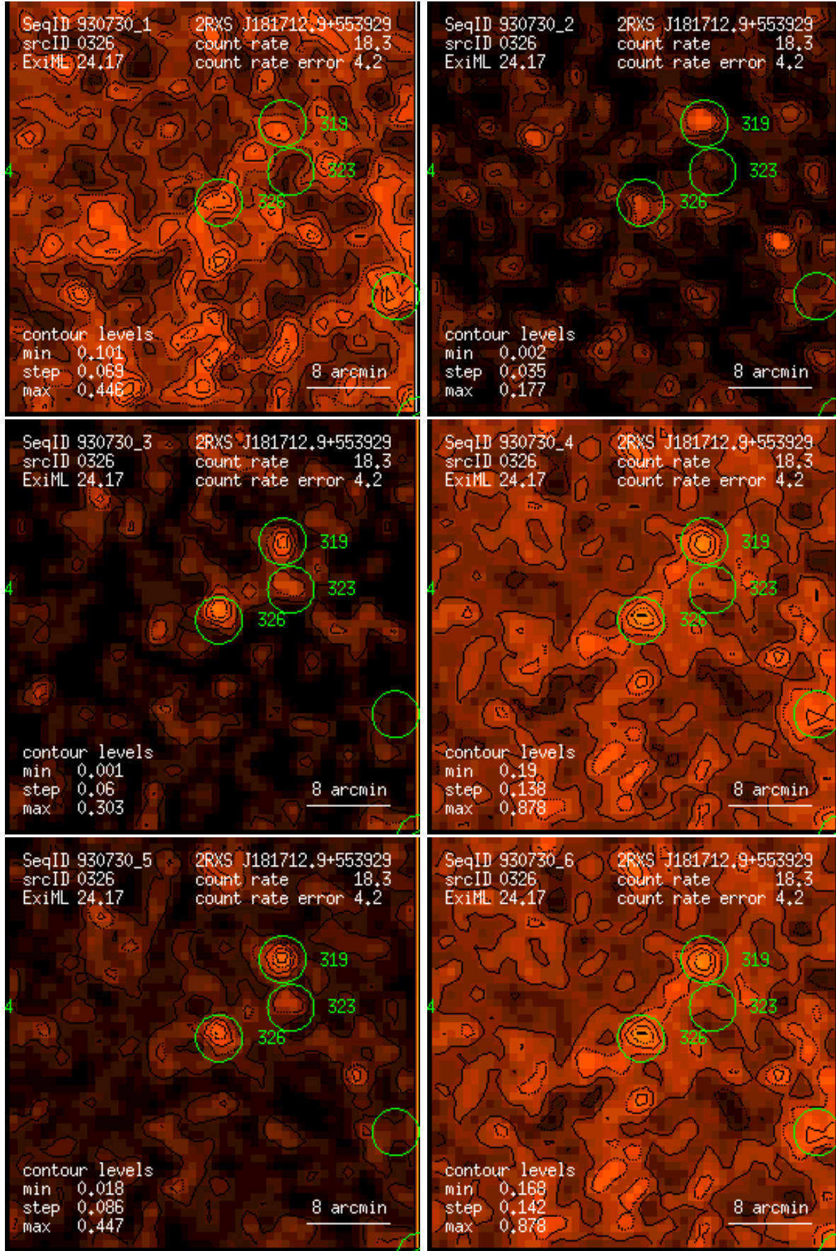
Figure 326: RASS 930730: detection 0326: band rate images, Gaussian filter: (1) PSPC channels 11 – 41, (2) 52 – 90, (3) 91 – 201, (4) 11 – 235, (5) 52 – 201, (6) 11 – 201. Broad band rates in counts/ks. Band rate contour levels in counts/ks/arcmin 2 .
