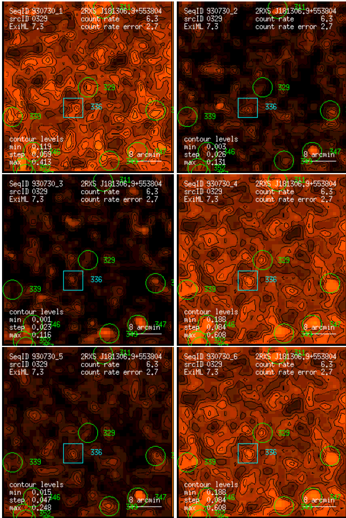
Figure 329: RASS 930730: detection 0329: band rate images, Gaussian filter: (1) PSPC channels 11 – 41, (2) 52 – 90, (3) 91 – 201, (4) 11 – 235, (5) 52 – 201, (6) 11 – 201. Broad band rates in counts/ks. Band rate contour levels in counts/ks/arcmin 2 .
