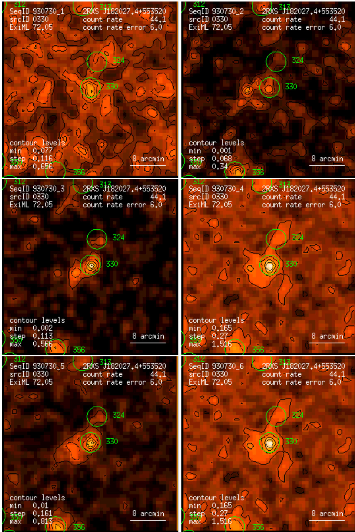
Figure 330: RASS 930730: detection 0330: band rate images, Gaussian filter: (1) PSPC channels 11 – 41, (2) 52 – 90, (3) 91 – 201, (4) 11 – 235, (5) 52 – 201, (6) 11 – 201. Broad band rates in counts/ks. Band rate contour levels in counts/ks/arcmin 2 .
