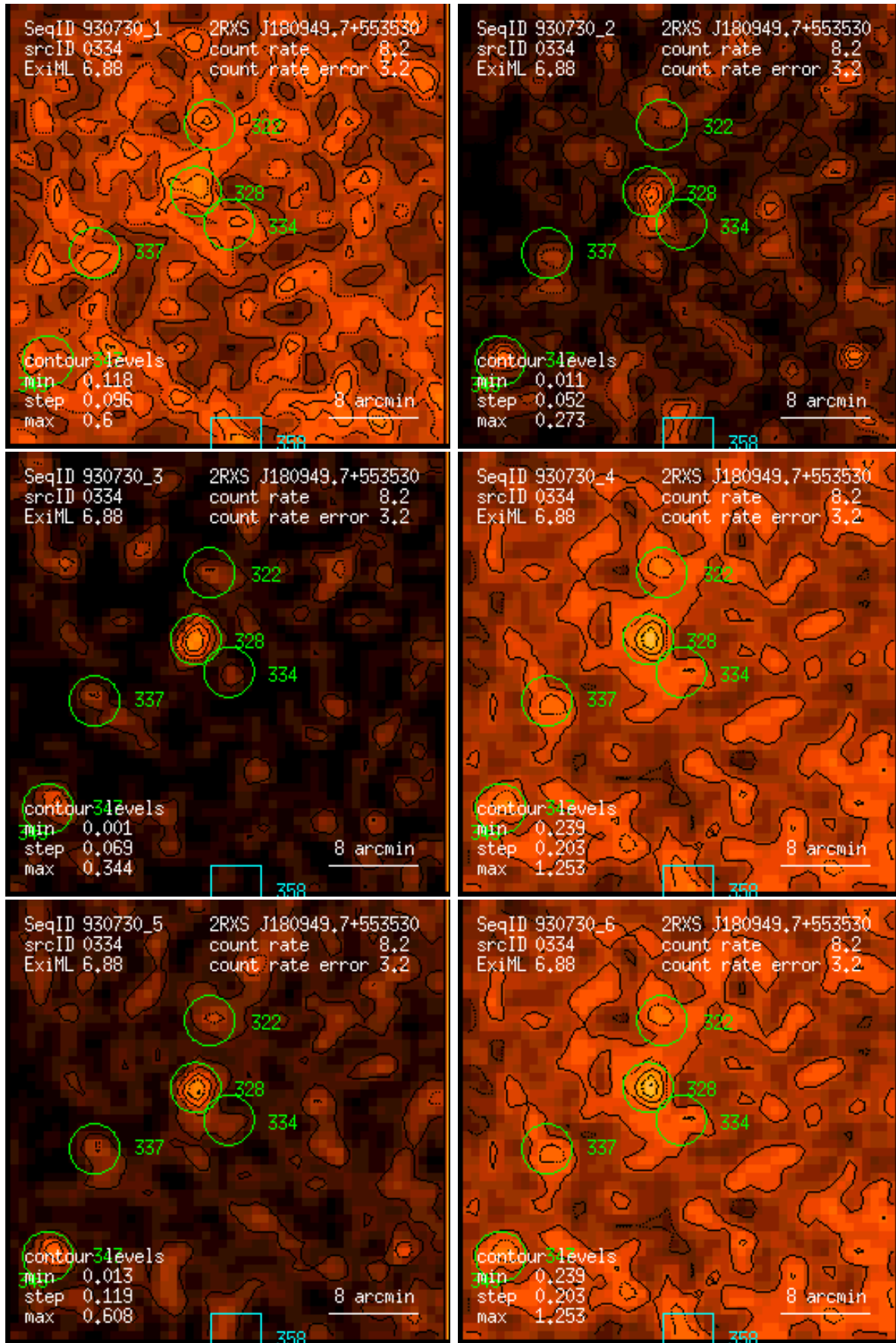
Figure 334: RASS 930730: detection 0334: band rate images, Gaussian filter: (1) PSPC channels 11 – 41, (2) 52 – 90, (3) 91 – 201, (4) 11 – 235, (5) 52 – 201, (6) 11 – 201. Broad band rates in counts/ks. Band rate contour levels in counts/ks/arcmin 2 .
