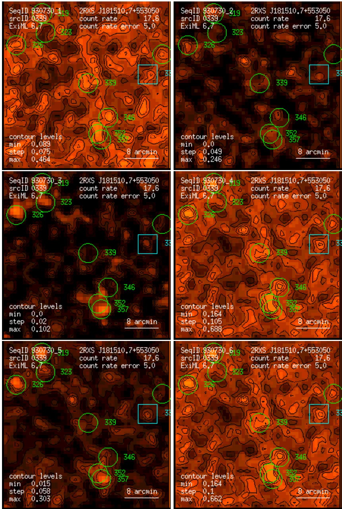
Figure 339: RASS 930730: detection 0339: band rate images, Gaussian filter: (1) PSPC channels 11 – 41, (2) 52 – 90, (3) 91 – 201, (4) 11 – 235, (5) 52 – 201, (6) 11 – 201. Broad band rates in counts/ks. Band rate contour levels in counts/ks/arcmin 2 .
