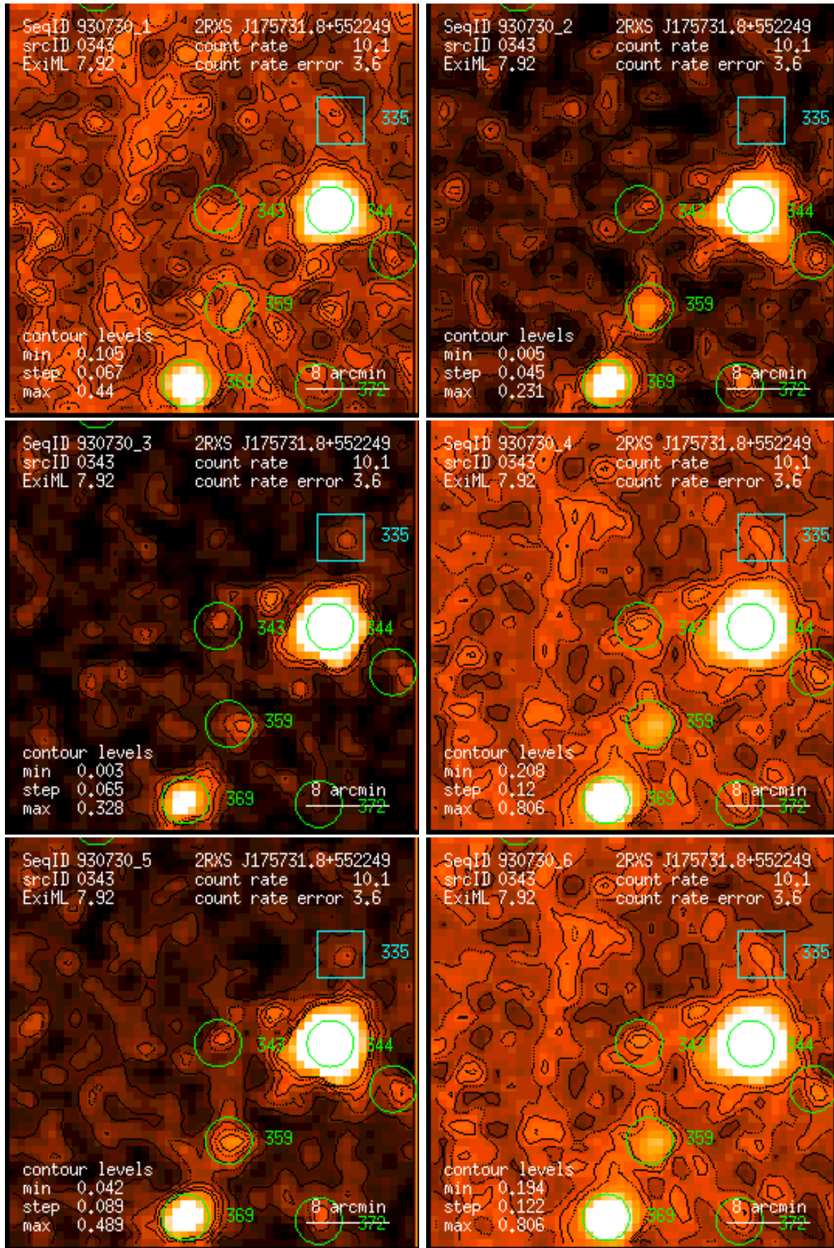
Figure 343: RASS 930730: detection 0343: band rate images, Gaussian filter: (1) PSPC channels 11 – 41, (2) 52 – 90, (3) 91 – 201, (4) 11 – 235, (5) 52 – 201, (6) 11 – 201. Broad band rates in counts/ks. Band rate contour levels in counts/ks/arcmin 2 .
