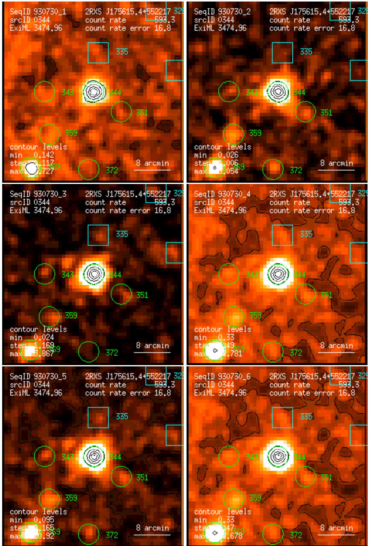
Figure 344: RASS 930730: detection 0344: band rate images, Gaussian filter: (1) PSPC channels 11 – 41, (2) 52 – 90, (3) 91 – 201, (4) 11 – 235, (5) 52 – 201, (6) 11 – 201. Broad band rates in counts/ks. Band rate contour levels in counts/ks/arcmin 2 .
