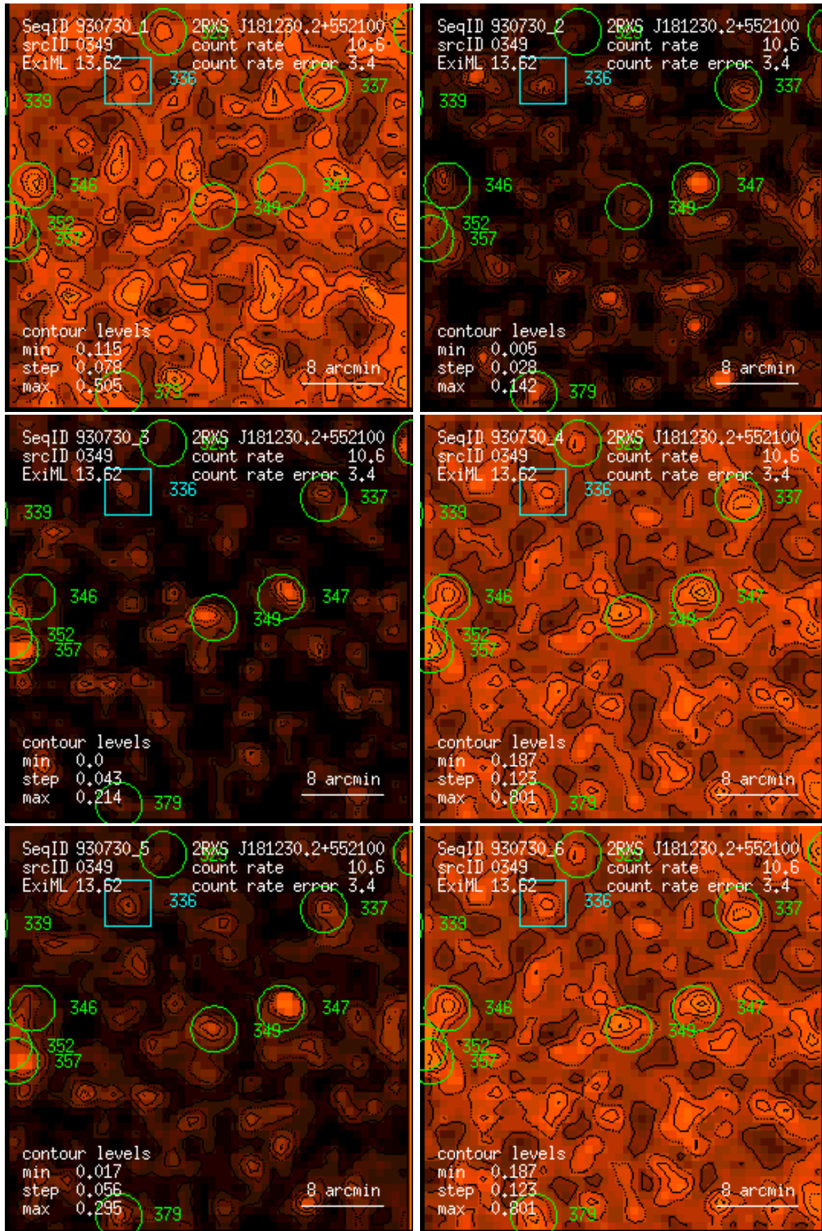
Figure 349: RASS 930730: detection 0349: band rate images, Gaussian filter: (1) PSPC channels 11 – 41, (2) 52 – 90, (3) 91 – 201, (4) 11 – 235, (5) 52 – 201, (6) 11 – 201. Broad band rates in counts/ks. Band rate contour levels in counts/ks/arcmin 2 .
