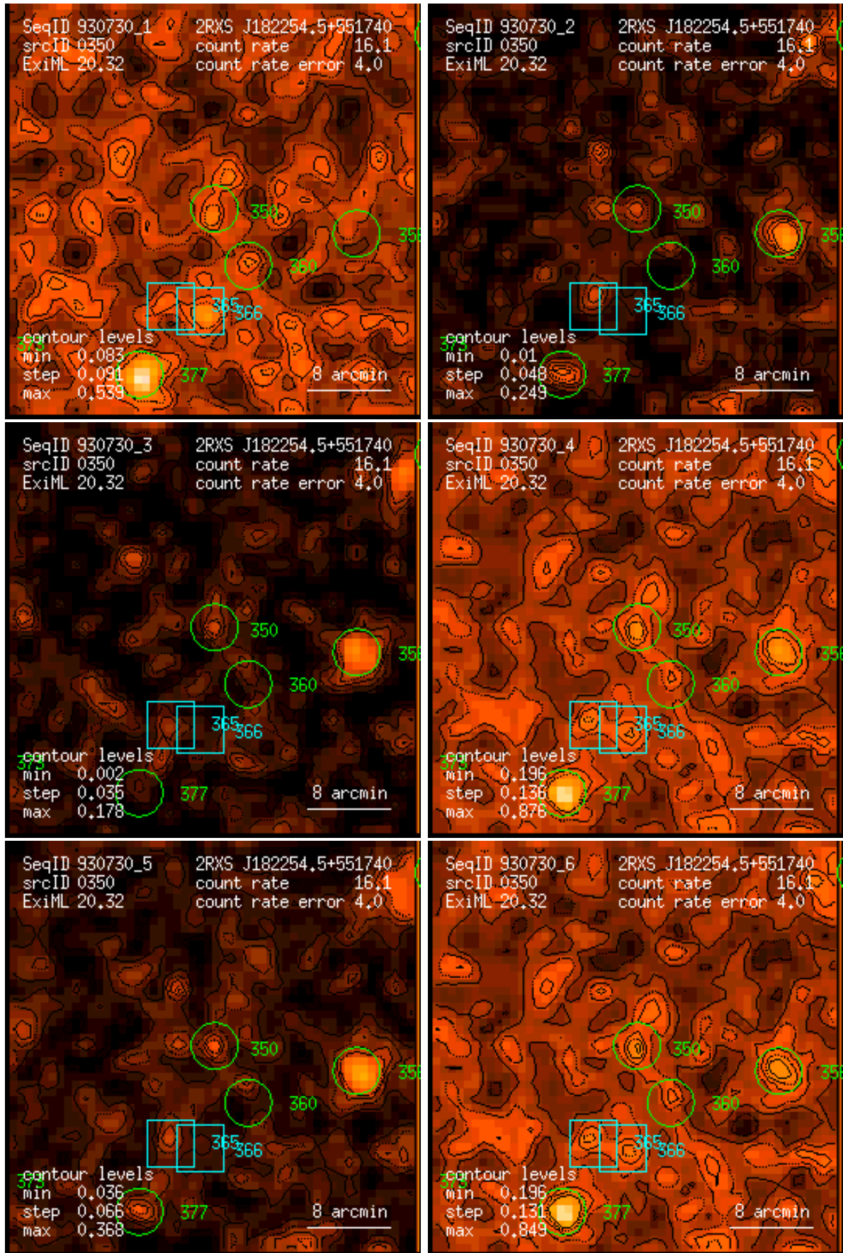
Figure 350: RASS 930730: detection 0350: band rate images, Gaussian filter: (1) PSPC channels 11 – 41, (2) 52 – 90, (3) 91 – 201, (4) 11 – 235, (5) 52 – 201, (6) 11 – 201. Broad band rates in counts/ks. Band rate contour levels in counts/ks/arcmin 2 .
