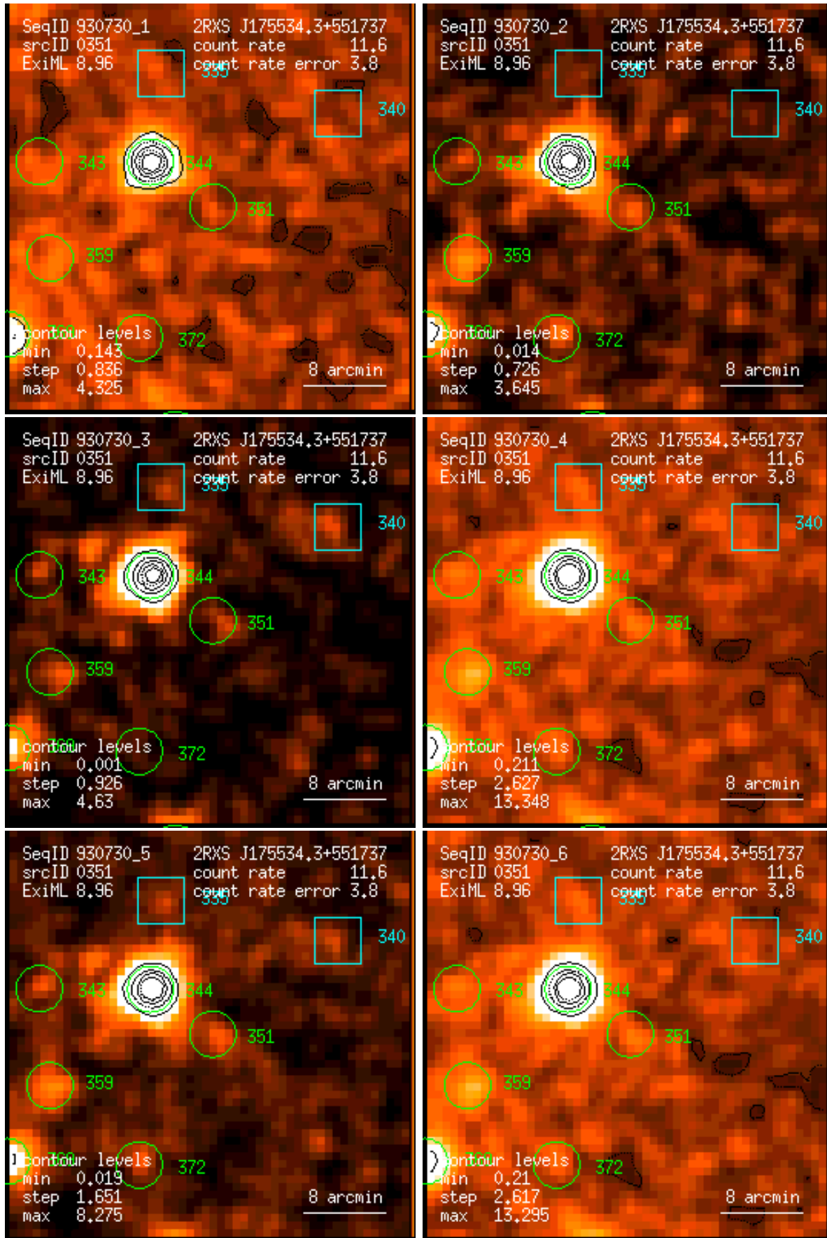
Figure 351: RASS 930730: detection 0351: band rate images, Gaussian filter: (1) PSPC channels 11 – 41, (2) 52 – 90, (3) 91 – 201, (4) 11 – 235, (5) 52 – 201, (6) 11 – 201. Broad band rates in counts/ks. Band rate contour levels in counts/ks/arcmin 2 .
