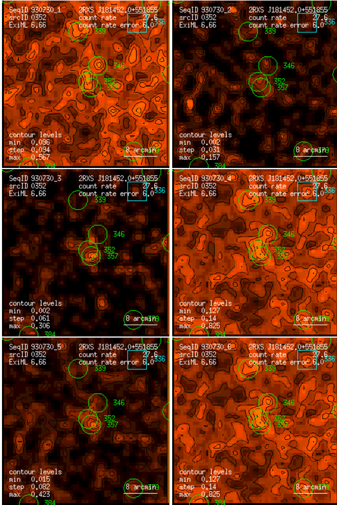
Figure 352: RASS 930730: detection 0352: band rate images, Gaussian filter: (1) PSPC channels 11 – 41, (2) 52 – 90, (3) 91 – 201, (4) 11 – 235, (5) 52 – 201, (6) 11 – 201. Broad band rates in counts/ks. Band rate contour levels in counts/ks/arcmin 2 .
