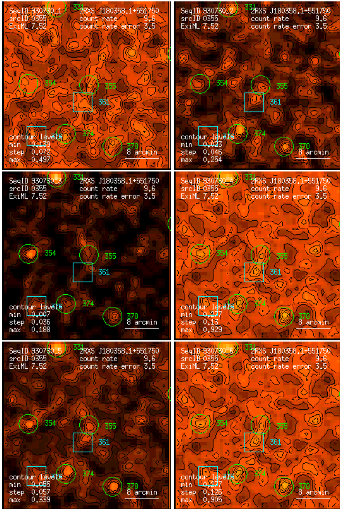
Figure 355: RASS 930730: detection 0355: band rate images, Gaussian filter: (1) PSPC channels 11 – 41, (2) 52 – 90, (3) 91 – 201, (4) 11 – 235, (5) 52 – 201, (6) 11 – 201. Broad band rates in counts/ks. Band rate contour levels in counts/ks/arcmin 2 .
