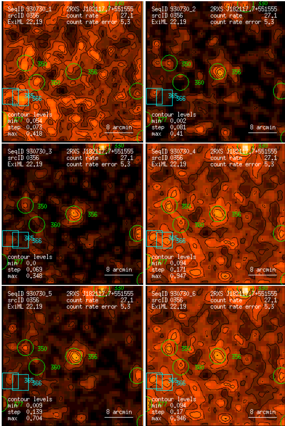
Figure 356: RASS 930730: detection 0356: band rate images, Gaussian filter: (1) PSPC channels 11 – 41, (2) 52 – 90, (3) 91 – 201, (4) 11 – 235, (5) 52 – 201, (6) 11 – 201. Broad band rates in counts/ks. Band rate contour levels in counts/ks/arcmin 2 .
