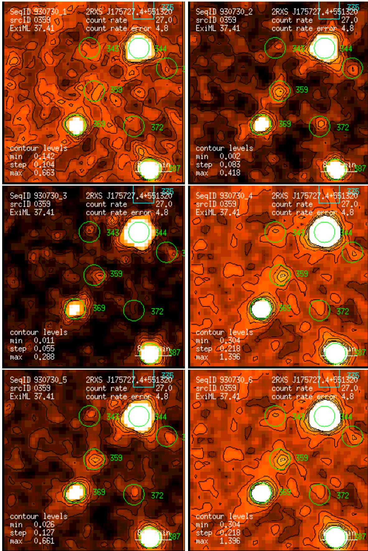
Figure 359: RASS 930730: detection 0359: band rate images, Gaussian filter: (1) PSPC channels 11 – 41, (2) 52 – 90, (3) 91 – 201, (4) 11 – 235, (5) 52 – 201, (6) 11 – 201. Broad band rates in counts/ks. Band rate contour levels in counts/ks/arcmin 2 .
