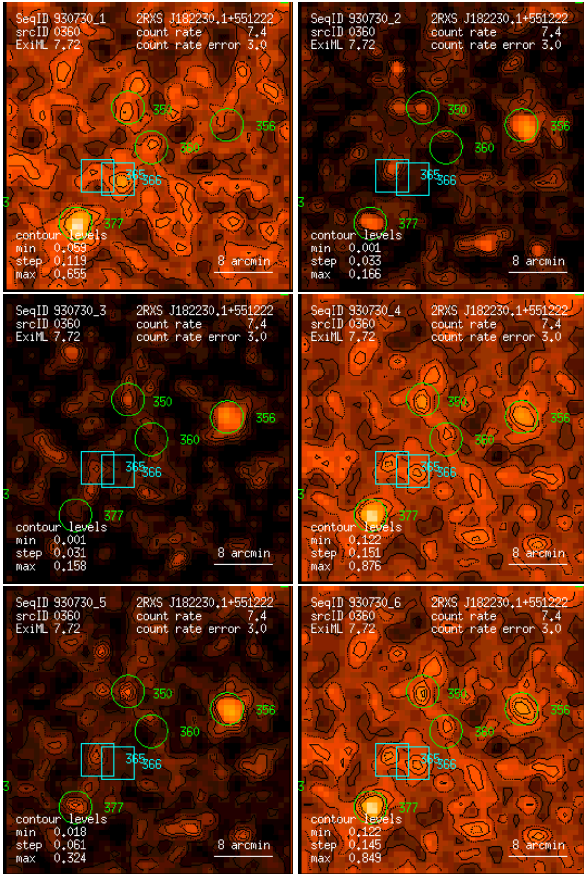
Figure 360: RASS 930730: detection 0360: band rate images, Gaussian filter: (1) PSPC channels 11 – 41, (2) 52 – 90, (3) 91 – 201, (4) 11 – 235, (5) 52 – 201, (6) 11 – 201. Broad band rates in counts/ks. Band rate contour levels in counts/ks/arcmin 2 .
