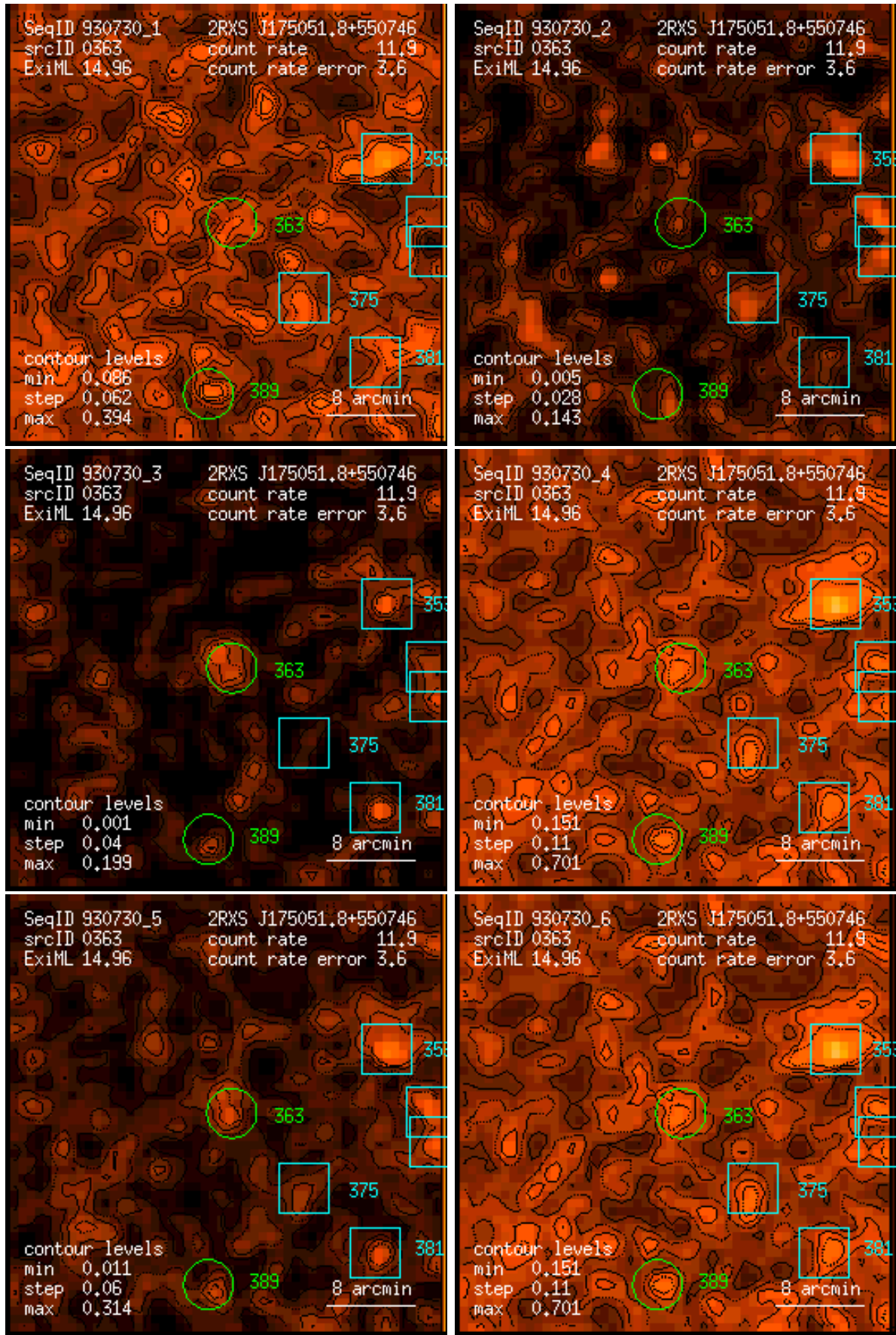
Figure 363: RASS 930730: detection 0363: band rate images, Gaussian filter: (1) PSPC channels 11 – 41, (2) 52 – 90, (3) 91 – 201, (4) 11 – 235, (5) 52 – 201, (6) 11 – 201. Broad band rates in counts/ks. Band rate contour levels in counts/ks/arcmin 2 .
