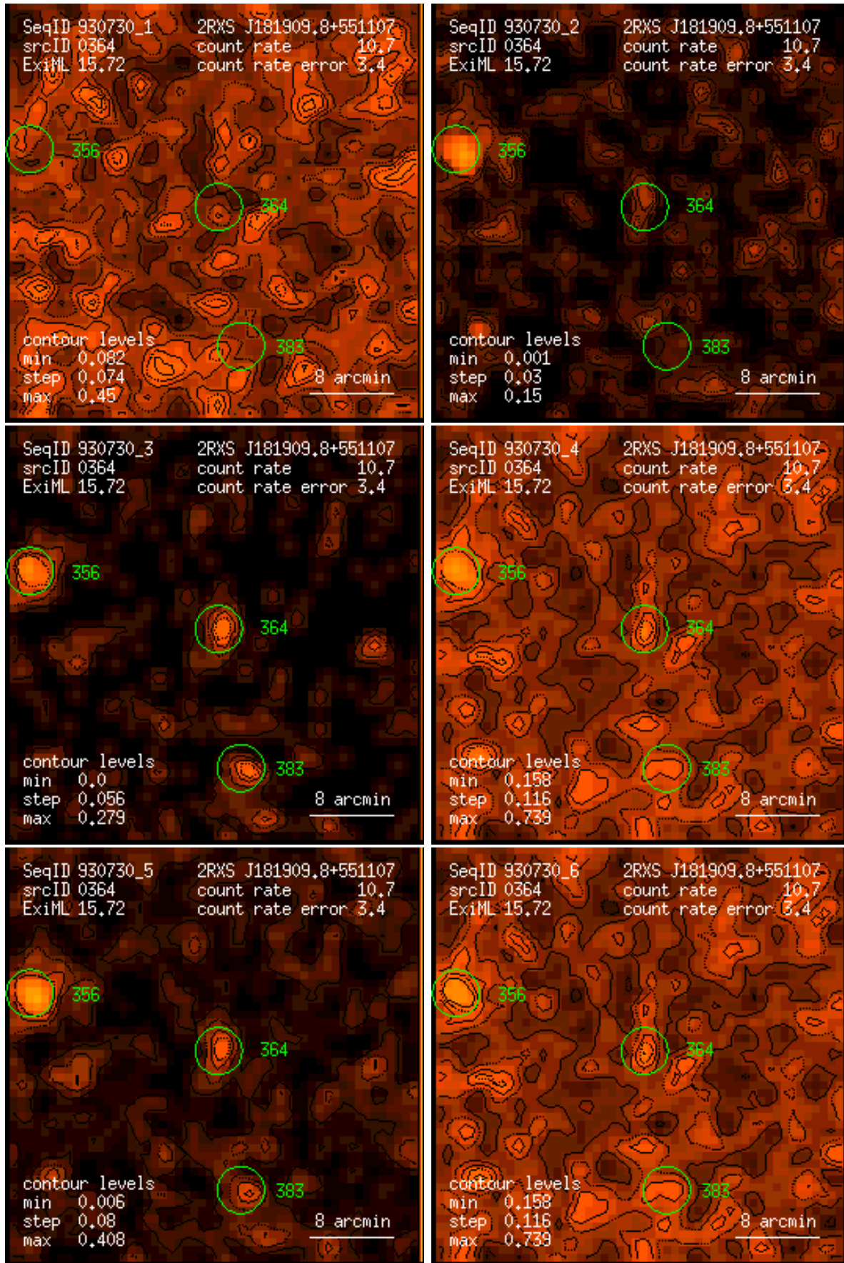
Figure 364: RASS 930730: detection 0364: band rate images, Gaussian filter: (1) PSPC channels 11 – 41, (2) 52 – 90, (3) 91 – 201, (4) 11 – 235, (5) 52 – 201, (6) 11 – 201. Broad band rates in counts/ks. Band rate contour levels in counts/ks/arcmin 2 .
