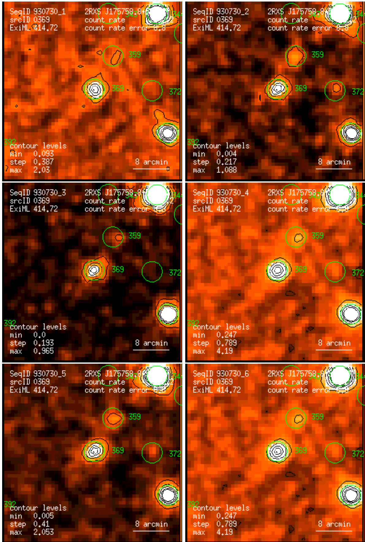
Figure 369: RASS 930730: detection 0369: band rate images, Gaussian filter: (1) PSPC channels 11 – 41, (2) 52 – 90, (3) 91 – 201, (4) 11 – 235, (5) 52 – 201, (6) 11 – 201. Broad band rates in counts/ks. Band rate contour levels in counts/ks/arcmin 2 .
