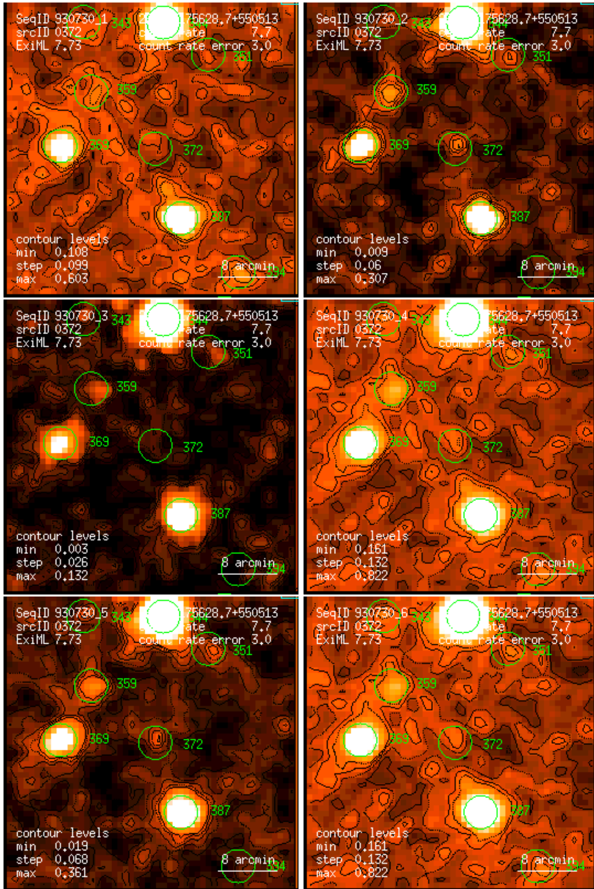
Figure 372: RASS 930730: detection 0372: band rate images, Gaussian filter: (1) PSPC channels 11 – 41, (2) 52 – 90, (3) 91 – 201, (4) 11 – 235, (5) 52 – 201, (6) 11 – 201. Broad band rates in counts/ks. Band rate contour levels in counts/ks/arcmin 2 .
