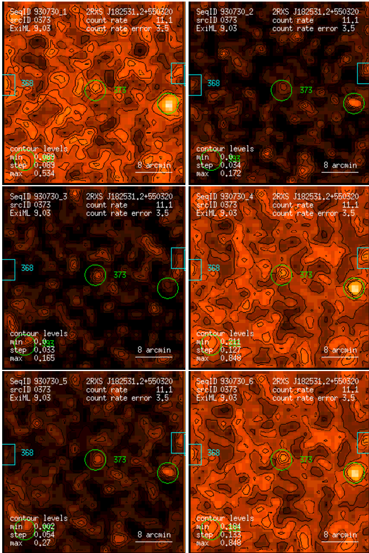
Figure 373: RASS 930730: detection 0373: band rate images, Gaussian filter: (1) PSPC channels 11 – 41, (2) 52 – 90, (3) 91 – 201, (4) 11 – 235, (5) 52 – 201, (6) 11 – 201. Broad band rates in counts/ks. Band rate contour levels in counts/ks/arcmin 2 .
