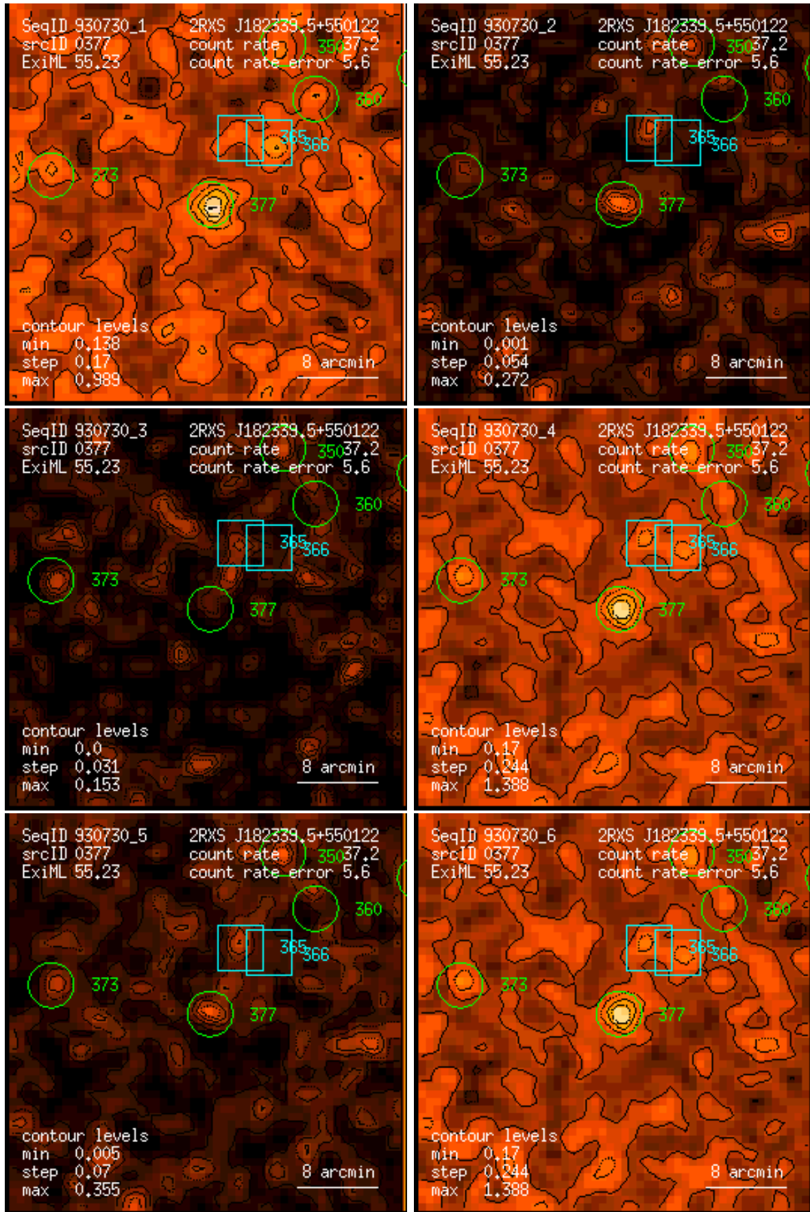
Figure 377: RASS 930730: detection 0377: band rate images, Gaussian filter: (1) PSPC channels 11 – 41, (2) 52 – 90, (3) 91 – 201, (4) 11 – 235, (5) 52 – 201, (6) 11 – 201. Broad band rates in counts/ks. Band rate contour levels in counts/ks/arcmin 2 .
